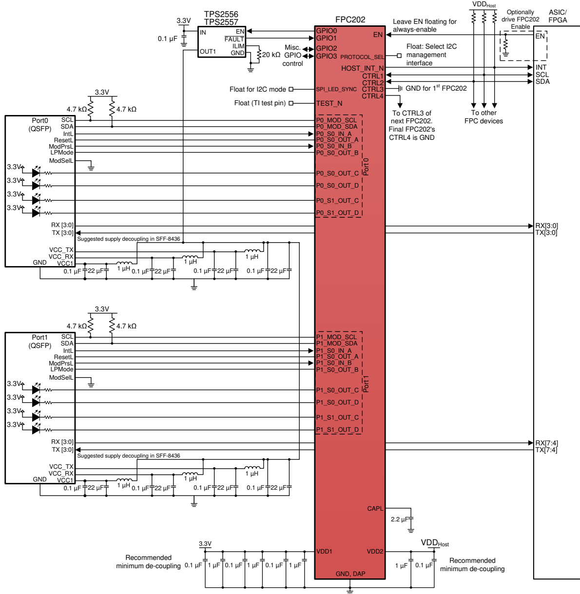
図 8-3. SFP/QSFP Application Schematic
