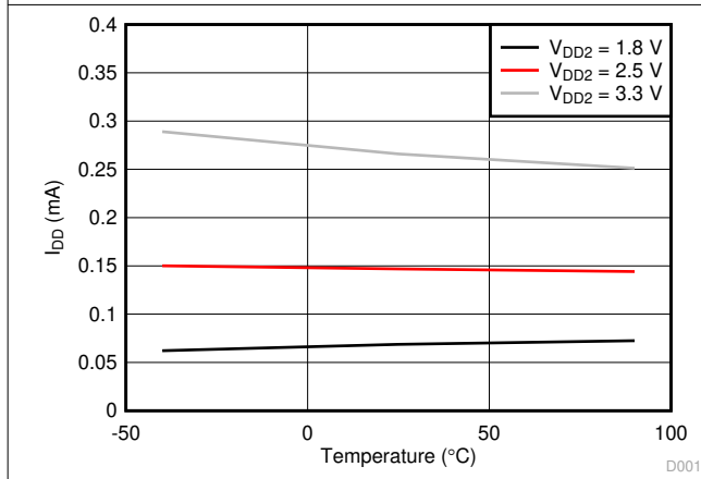
7-3. Static IDD2 vs. Ambient Temperature
