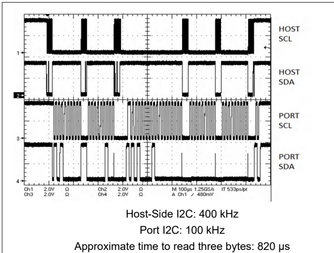
9-4. Downstream Read – Three Bytes Outside of Prefetched Range
