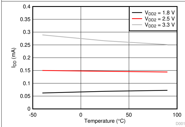
7-3. Static IDD2 vs. Ambient Temperature
