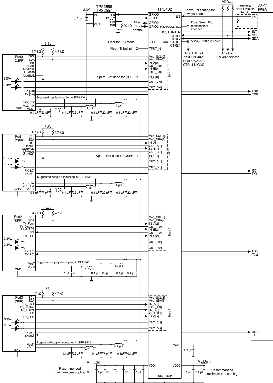
9-3. SFP/QSFP Application Schematic
