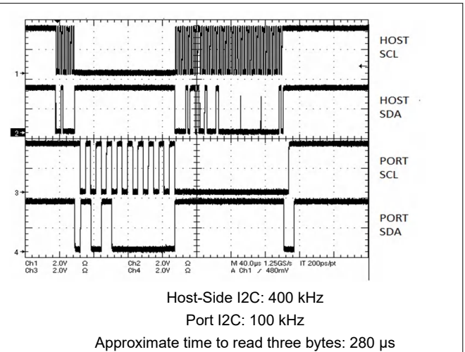
9-5. Downstream Read – Three Bytes in the Prefetched Range
