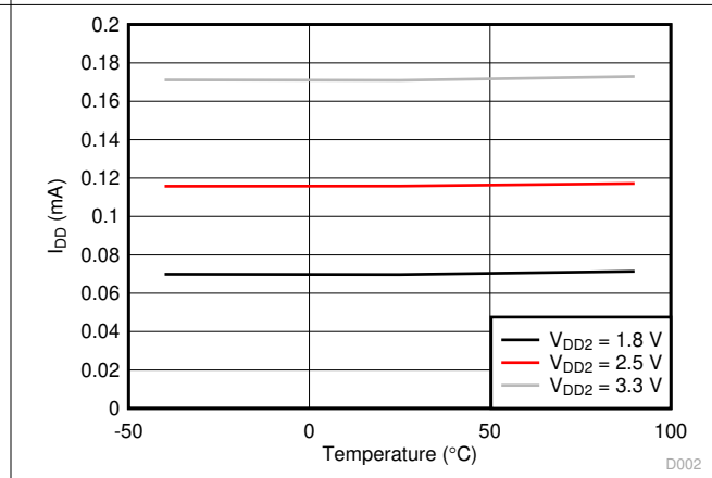
7-4. Dynamic IDD2 vs. Ambient Temperature
