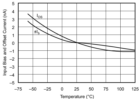
7-14. Input Bias and Offset Current vs Temperature
