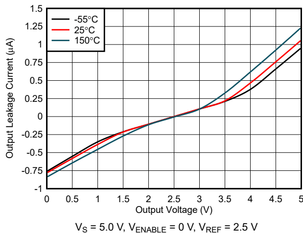
FIG 6-31. Output Leakage vs. Output Voltage (A1, A2, and A3 Devices)
