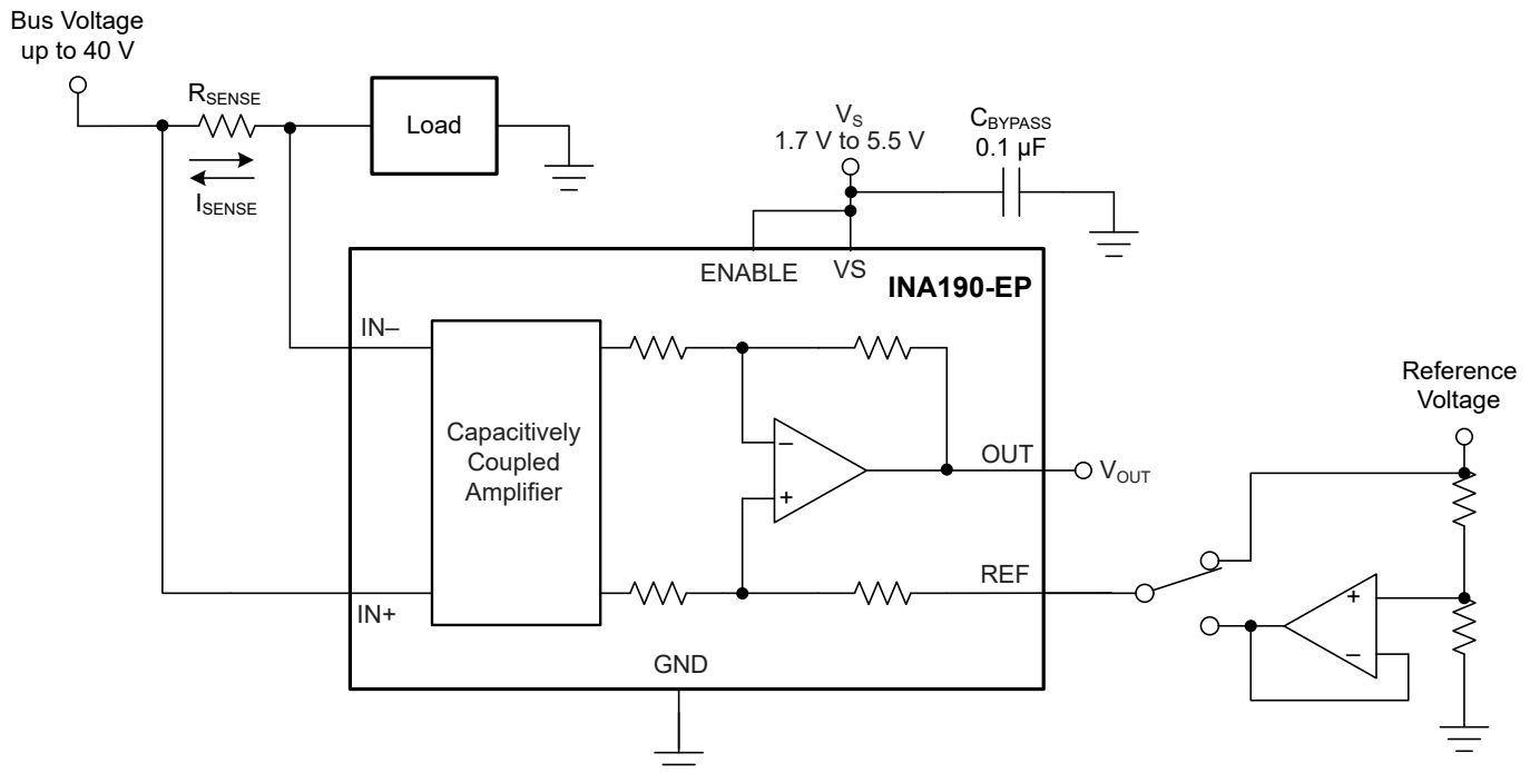
FIG 7-4. Bidirectional Application
