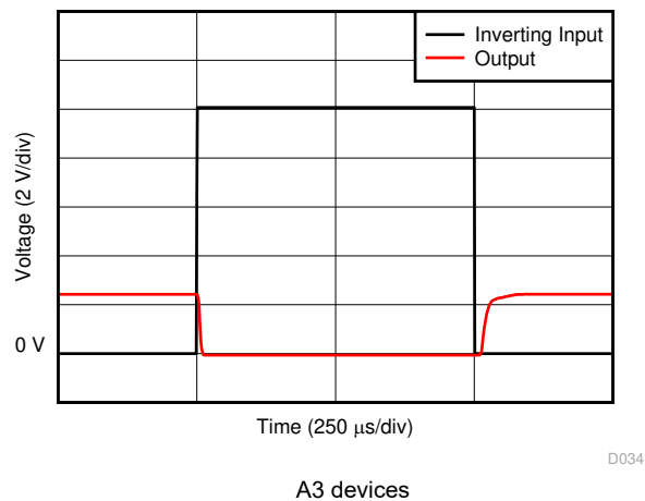
6-24. Inverting Differential Input Overload
