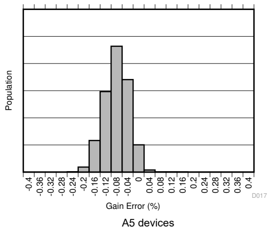
FIG 6-7. Gain Error Production Distribution
