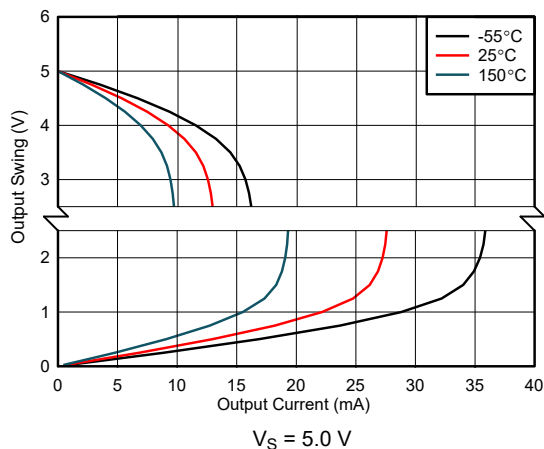
FIG 6-13. Output Voltage Swing vs. Output Current
