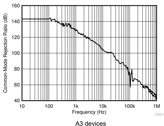
FIG 6-11. Common-Mode Rejection Ratio vs. Frequency
