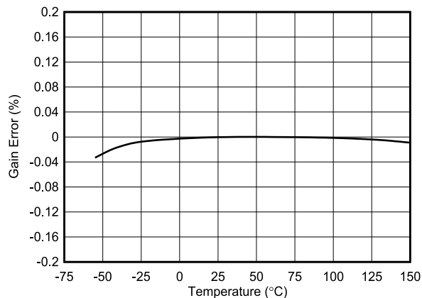
FIG 6-8. Gain Error vs. Temperature
