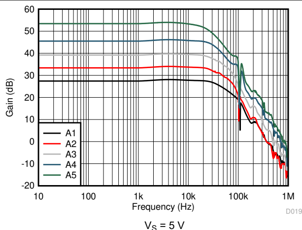
FIG 6-9. Gain vs. Frequency
