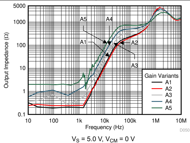
FIG 6-33. Output Impedance vs. Frequency
