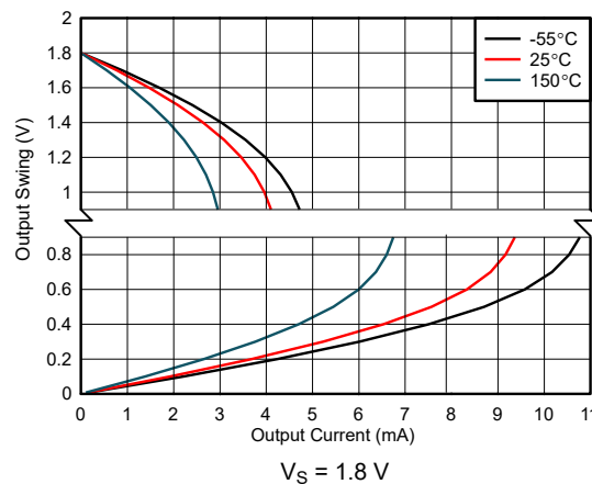
FIG 6-12. Output Voltage Swing vs. Output Current
