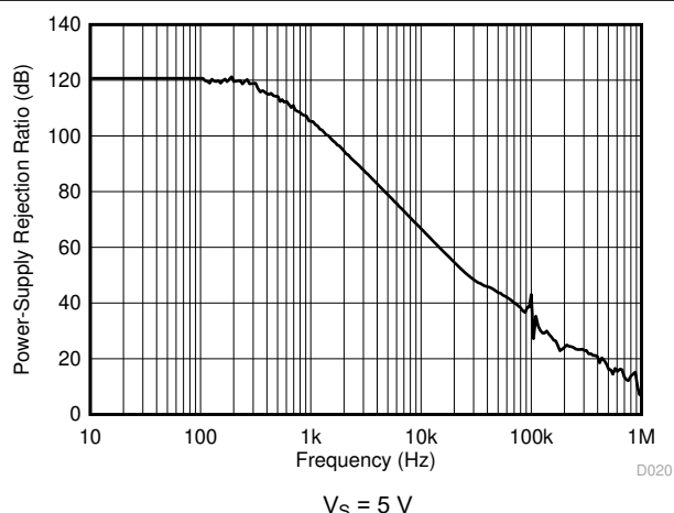
FIG 6-10. Power-Supply Rejection Ratio vs. Frequency
