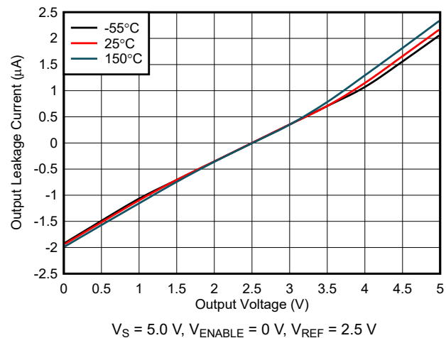
FIG 6-32. Output Leakage vs. Output Voltage (A4 and A5 Devices)
