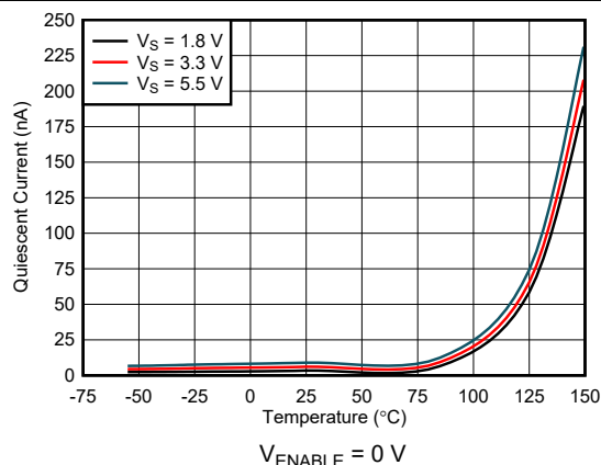
FIG 6-18. Quiescent Current vs. Temperature (Disabled)
