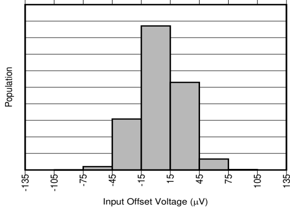
6-1. INA310A1 Input Offset Production Distribution
