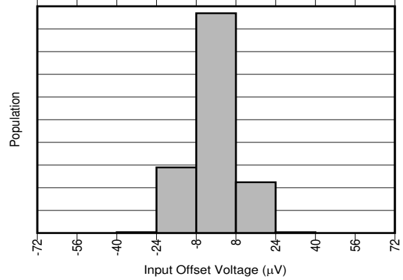
6-2. INA310A2 Input Offset Production Distribution
