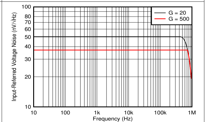
6-24. Input Referred Noise vs Frequency
