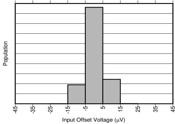
6-3. INA310A3 Input Offset Production Distribution
