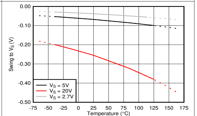
6-22. Swing to Supply vs Temperature
