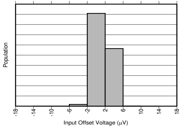
6-5. INA310A5 Input Offset Production Distribution
