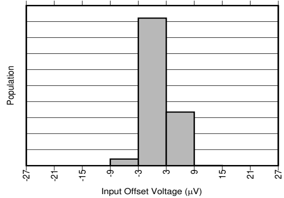
6-4. INA310A4 Input Offset Production Distribution
