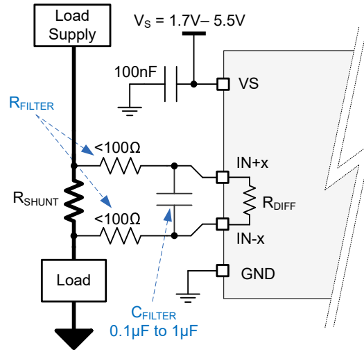
Figure 8-1. Input Filtering
