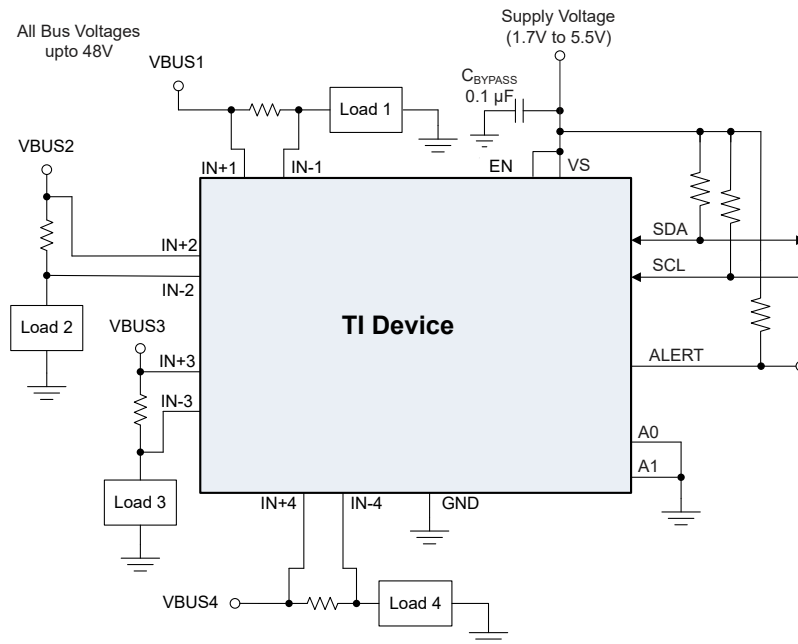
☒ 8-2. Typical High-Side Sensing Circuit Configuration, INA4235
