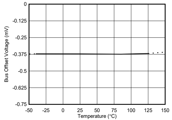
5-11. Bus Offset Voltage ( V_{IN-} ) vs. Temperature
