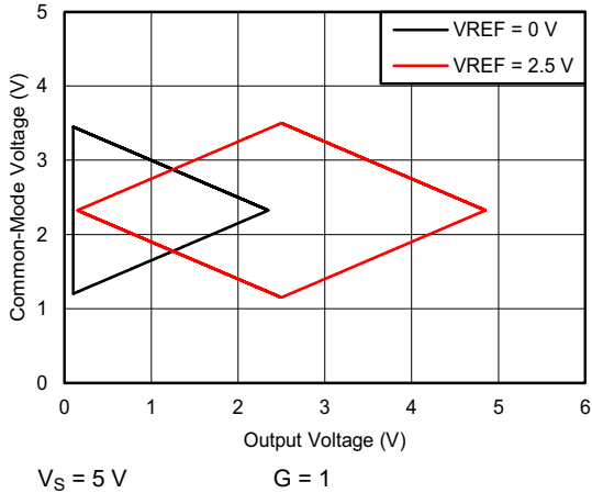
7-51. Input Common-Mode Voltage vs Output Voltage
