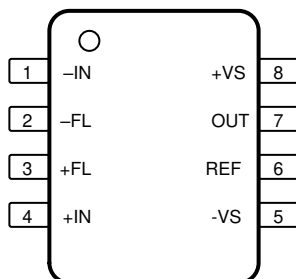
6-1. D Package, 8-Pin SOIC, Top View
