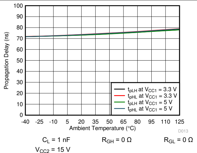
7-26. Propagation Delay vs Temperature
