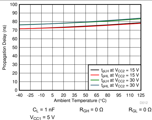
7-25. Propagation Delay vs Temperature
