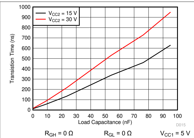
7-28. t_r Rise Time vs Load Capacitance
