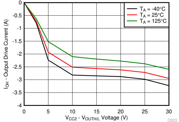
7-5. Output High Drive Current vs Output Voltage
