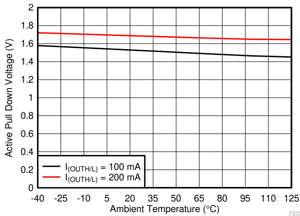
7-39. Active Pulldown Voltage vs Temperature
