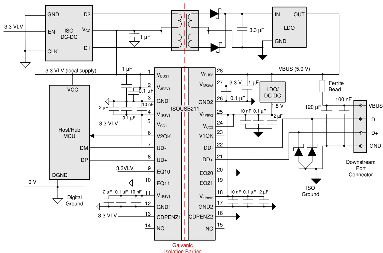
☒ 8-1. Isolated Host or Hub with ISOUSB211-Q1
