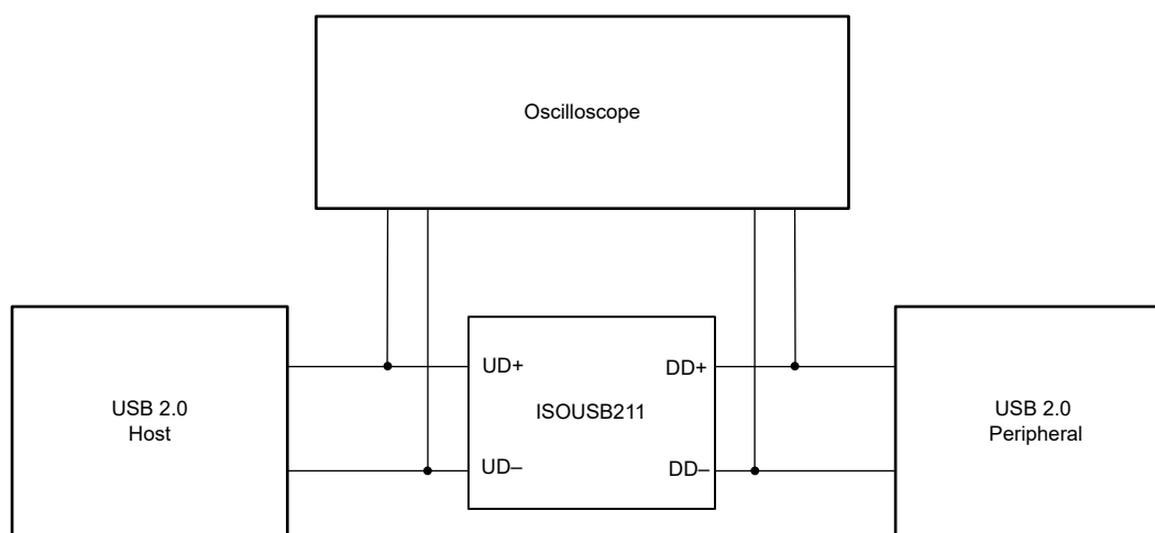
図 6-2. Upstream and Downstream Packet Parameter and Eye-Diagram Measurements for LS, FS
