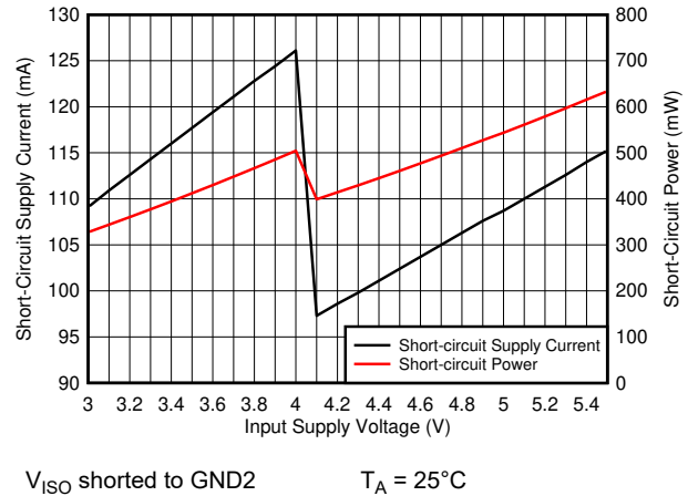
7-10. Short-Circuit Supply Current ( I_{SCC} ) and Power (P) vs Supply Voltage ( V_{CC} )
