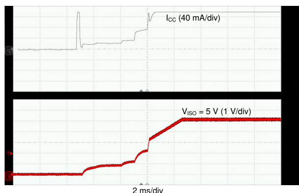
☒ 7-19. Soft Start at 120-mA Load
