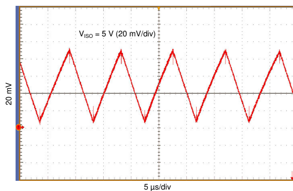
☒ 7-20. Soft Start at 10-mA Load
