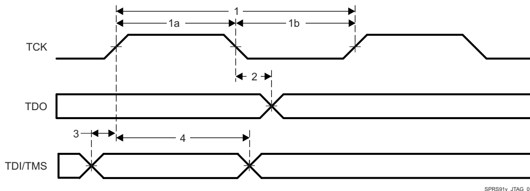
Figure 7-22. JTAG Timing
