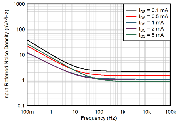
6-14. Input-Referred Noise Density vs Frequency
