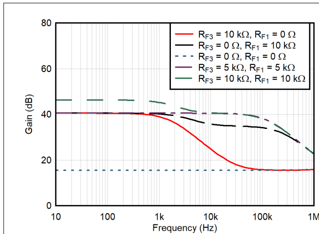
Figure 9-8. Gain/Phase
