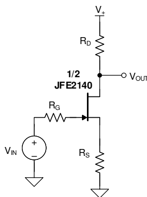
Figure 9-3. Common-Source Amplifier
