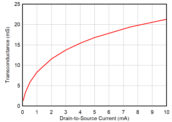
Figure 6-4. Common Source Transconductance vs Drain-to-Source Current
