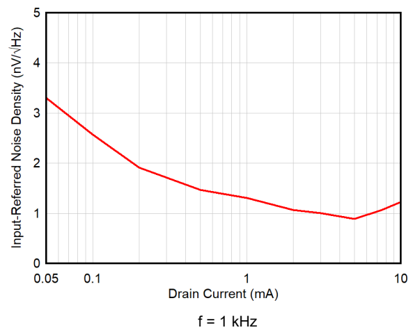
6-16. Input-Referred Noise Spectral Density vs Drain-to-Source Current
