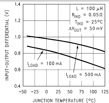
Figure 6. Dropout Voltage
