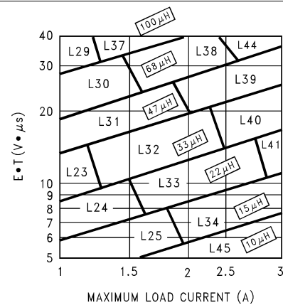
Figure 17. LM2673-ADJ
