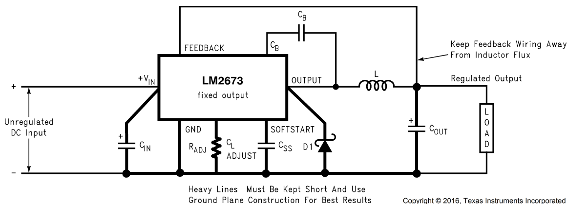
Figure 18. Basic Circuit for Fixed Output Voltage Applications
