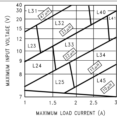
Figure 15. LM2673-5
