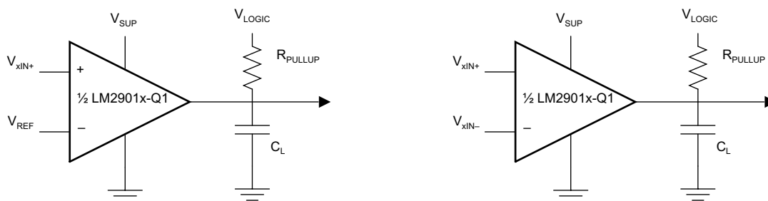
図 7-1. Single-Ended and Differential Comparator Configurations
