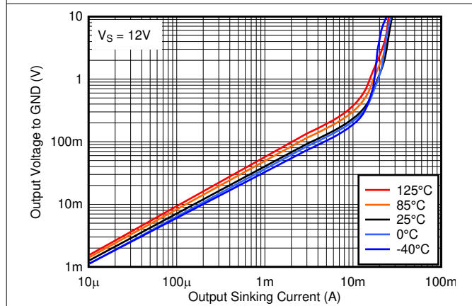
Fig 5-21. Output Low Voltage vs. Output Sinking Current at 12V
