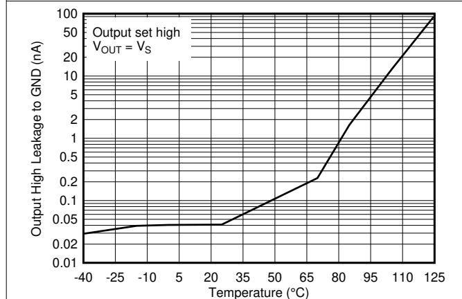
Fig 5-23. Output High Leakage Current vs. Temperature at 5V
