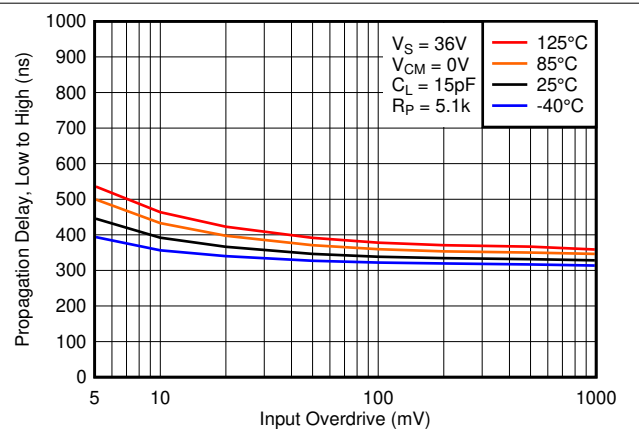
5-30. Low to High Propagation Delay vs. Input Overdrive Voltage, 36V
