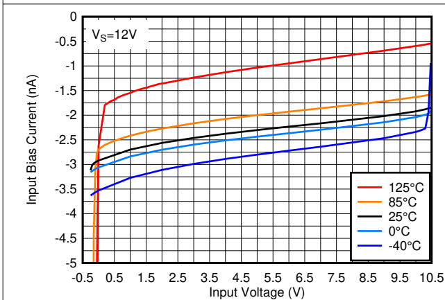
5-17. Input Bias Current vs. Input Voltage at 12V
