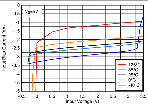
5-16. Input Bias Current vs. Input Voltage at 5V
