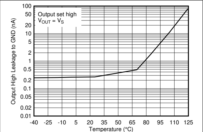
Fig 5-24. Output High Leakage Current vs. Temperature at 36V
