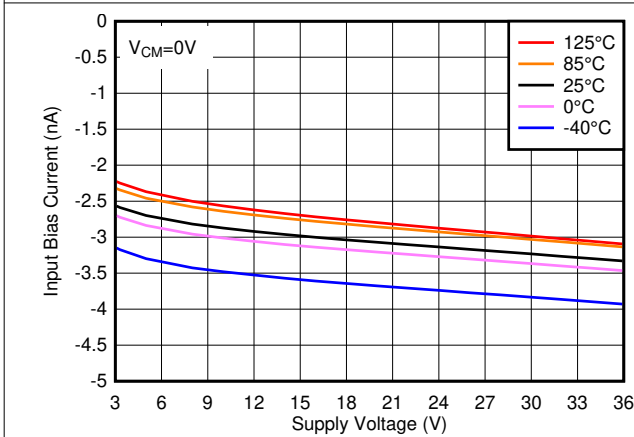
5-15. Input Bias Current vs. Supply Voltage
