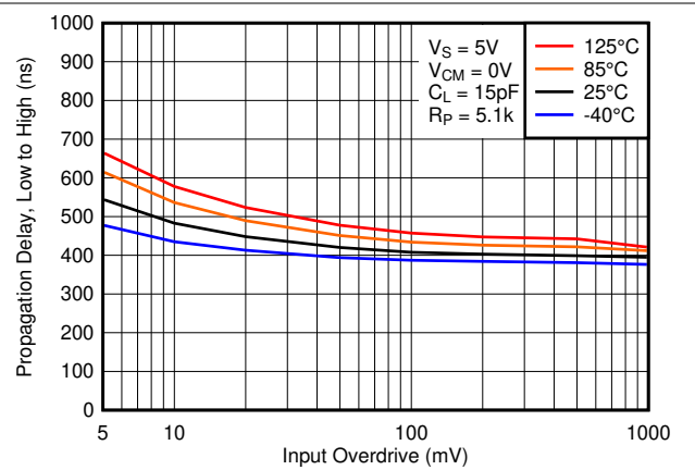
5-26. Low to High Propagation Delay vs. Input Overdrive Voltage, 5V
