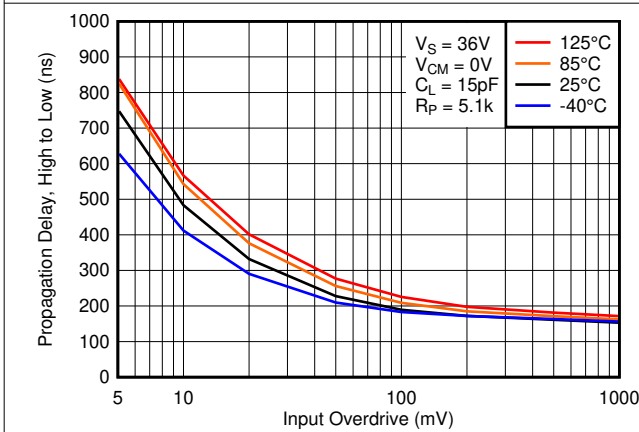
5-29. High to Low Propagation Delay vs. Input Overdrive Voltage, 36V
