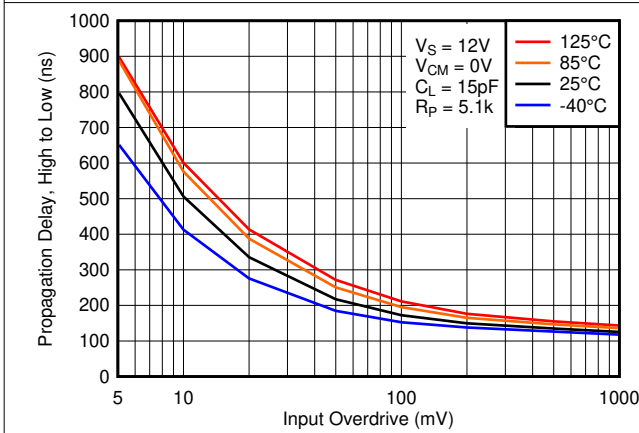
5-27. High to Low Propagation Delay vs. Input Overdrive Voltage, 12V
