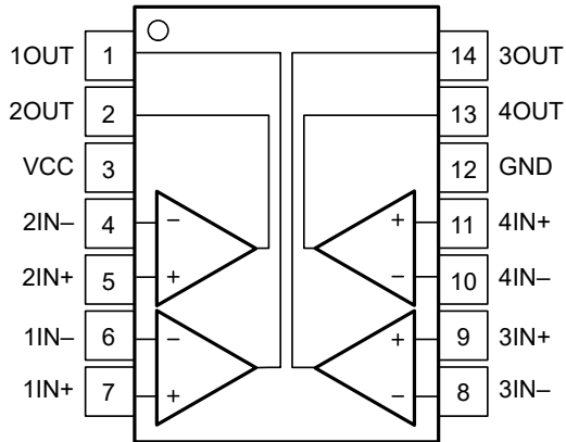
4-1. D, PW and DYY Packages 14-Pin SOIC, TSSOP and SOT-23 Top View
