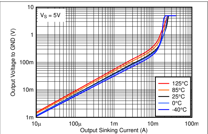
Fig 5-20. Output Low Voltage vs. Output Sinking Current at 5V
