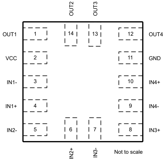
4-3. RUC Package 14-Pad X2QFN Top View
