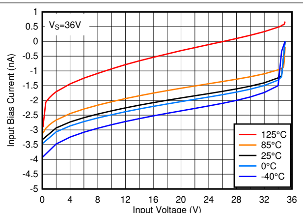
5-18. Input Bias Current vs. Input Voltage at 36V
