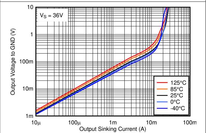
Fig 5-22. Output Low Voltage vs. Output Sinking Current at 36V
