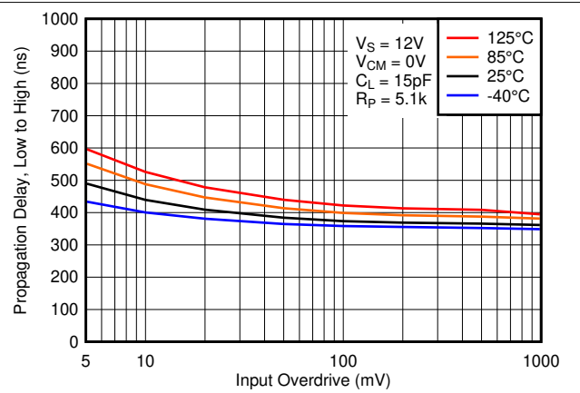
5-28. Low to High Propagation Delay vs. Input Overdrive Voltage, 12V
