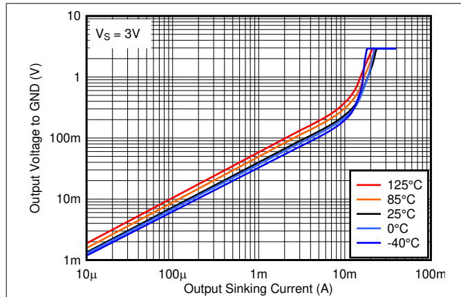
Fig 5-19. Output Low Voltage vs. Output Sinking Current at 3V
