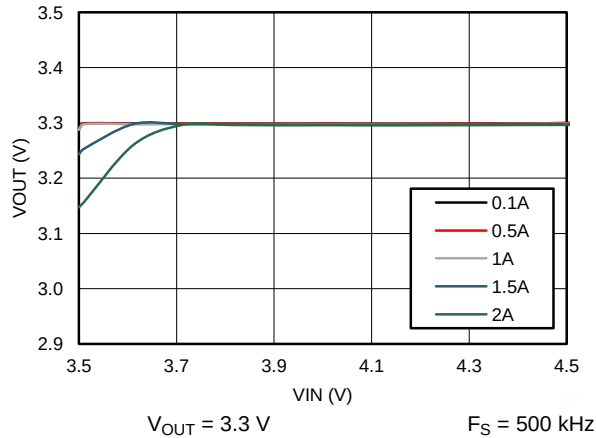
Figure 45. Dropout Voltage
