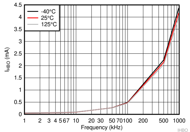
6-3. HB Quiescent Current
