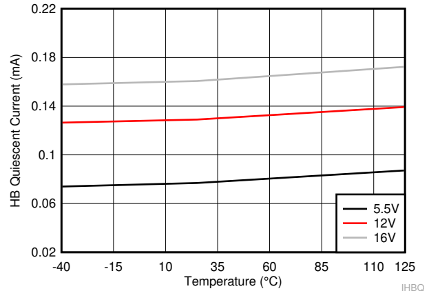
6-3. HB Quiescent Current
