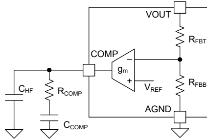
Figure 7-1. Type II g_m Amplifier Compensation
