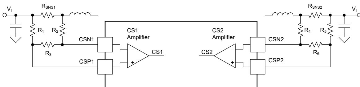
Figure 6-12. Peak Limit adjustment through additional resistors
