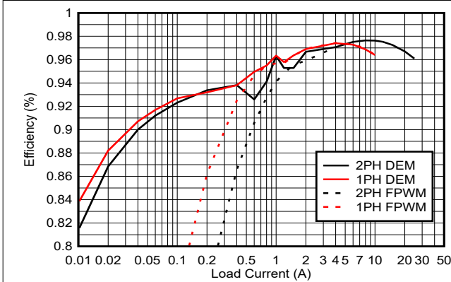
Figure 7-11. Efficiency vs Output Current, V_{in} = 14.4V , V_{out} = 24V
