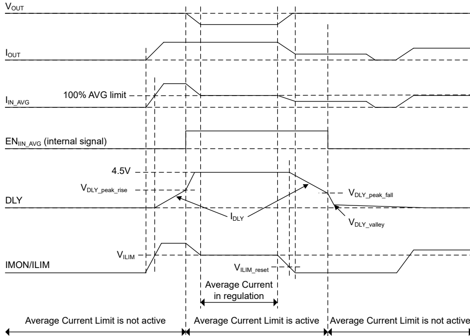
Figure 6-13. Average Current Limit
