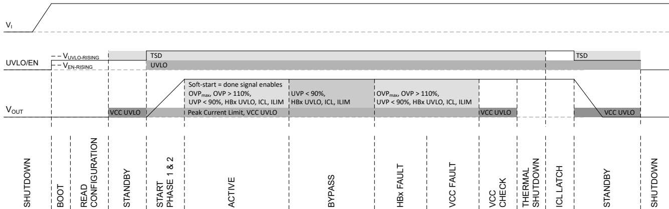
Figure 6-10. Protections
