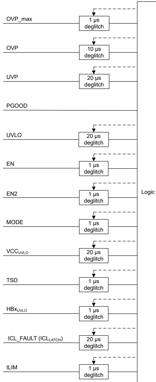
Figure 6-14. Signal Deglitching
