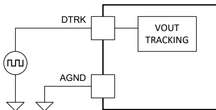
Figure 6-9. V_{OUT} Tracking by Digital Signal
