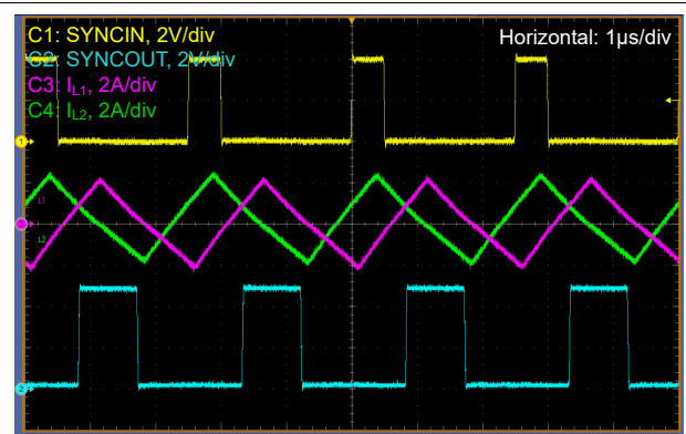
Figure 7-19. V_{in} = 14.4V , V_{out} = 24V , FPWM, I_{load} = 0A , CFG2 = Level 11
