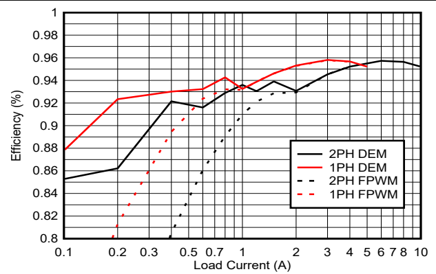
Figure 7-12. Efficiency vs Output Current, V_{in} = 14.4V , V_{out} = 45V
