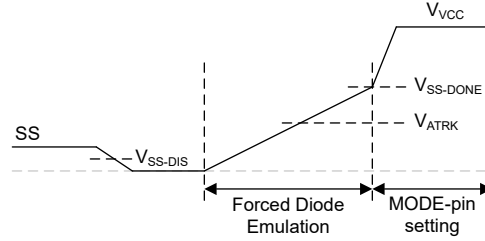
Figure 6-6. Soft Start
