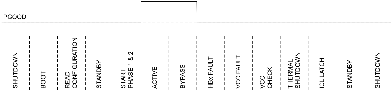
Figure 6-11. PGOOD Status for All Device States
