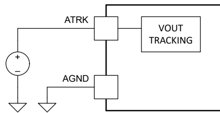
Figure 6-8. V_{OUT} Tracking by Analog Voltage
