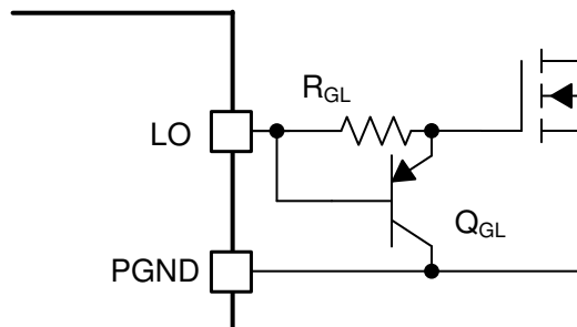
Figure 6-15. Slew Rate Control
