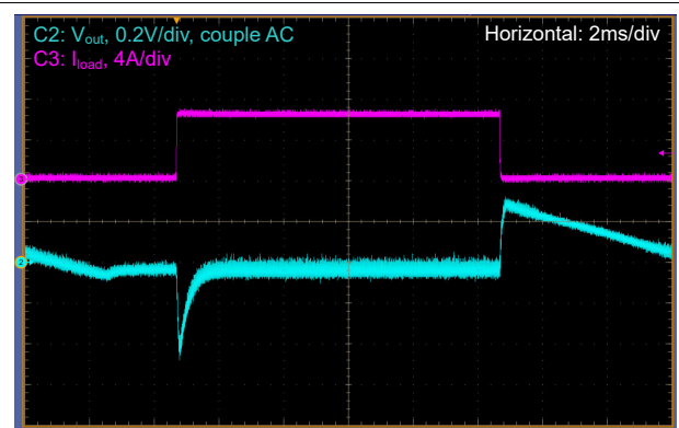
Figure 7-17. Load Transient, V_{in} = 14.4V , V_{out} = 24V , DEM, I_{load} = 0A to 6.25A at 1A/\mu s
