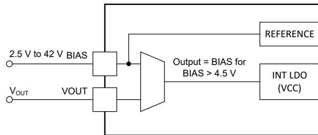
Figure 6-5. On the Fly BIAS Supply Selection
