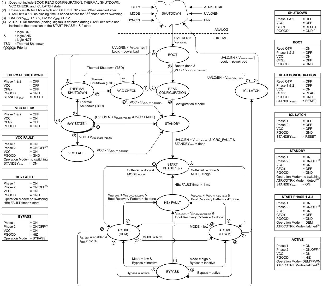
Figure 6-16. Functional State Diagram
