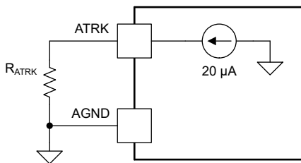
Figure 6-7. V_{OUT} Programming by Resistor
