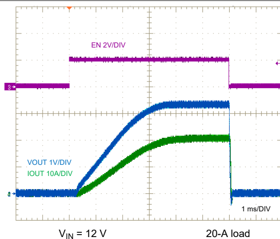
9-44. ENABLE ON and OFF Characteristic
