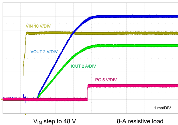
9-23. Start-Up Characteristic
