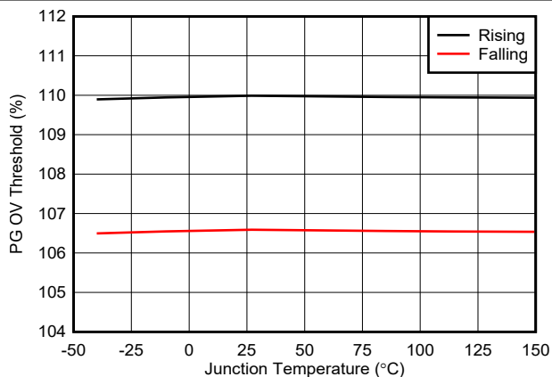
7-10. PG OV Thresholds vs Temperature
