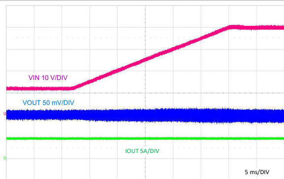
9-32. Full load Switching
