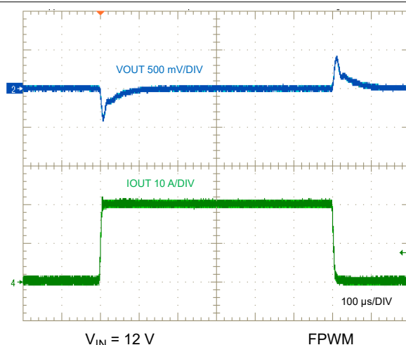
9-46. Load Transient, 0 A to 20 A
