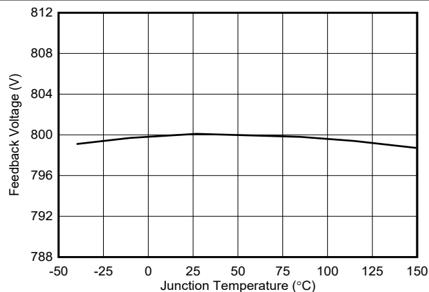
7-9. Feedback (FB) Voltage vs Temperature
