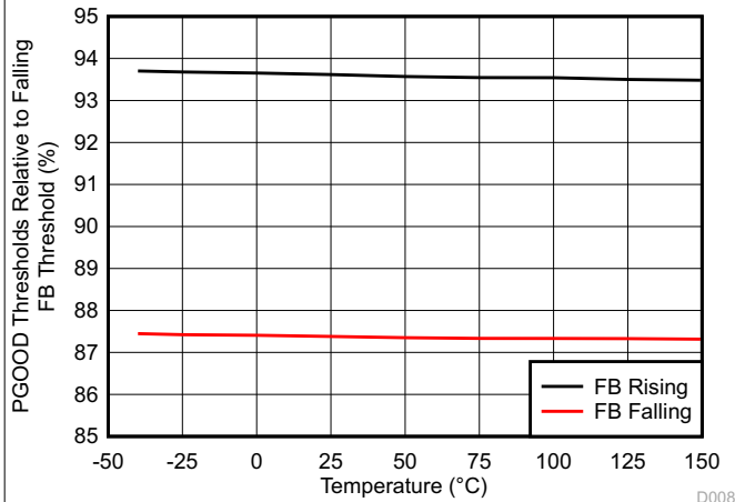
6-13. PGOOD Thresholds vs Temperature
