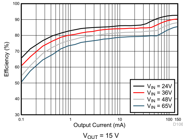
FIG 8-30. Efficiency
