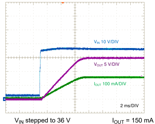
FIG 8-31. Start-Up, Full Load
