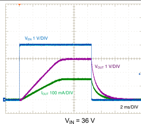
FIG 8-34. Enable ON and OFF
