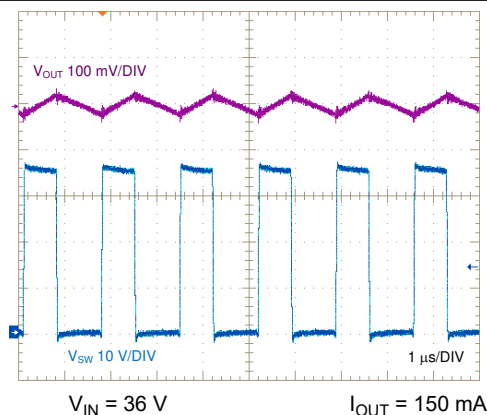
FIG 8-32. SW Node and Output Ripple Voltage, Full Load
