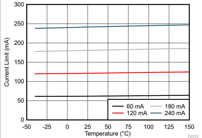
6-14. Peak Current Limits vs Temperature
