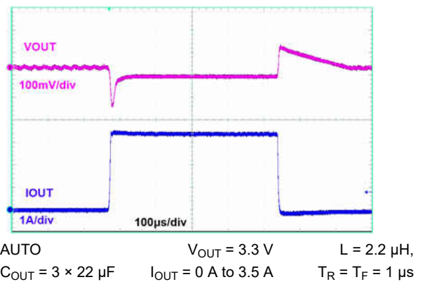
9-30. Load Transient
