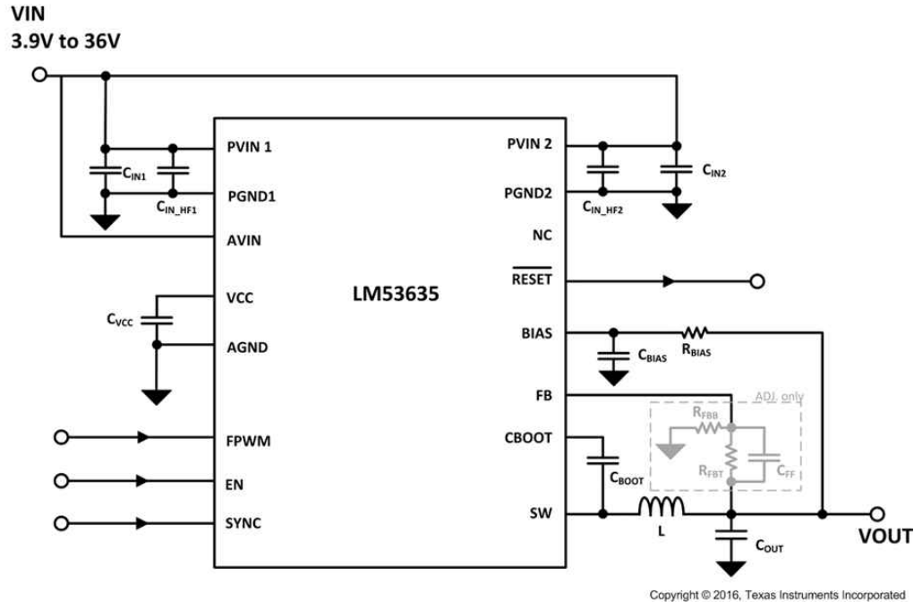
☒ 9-1. General Application Circuit
