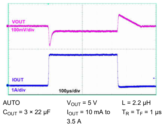
Figure 9-16. Load Transients
