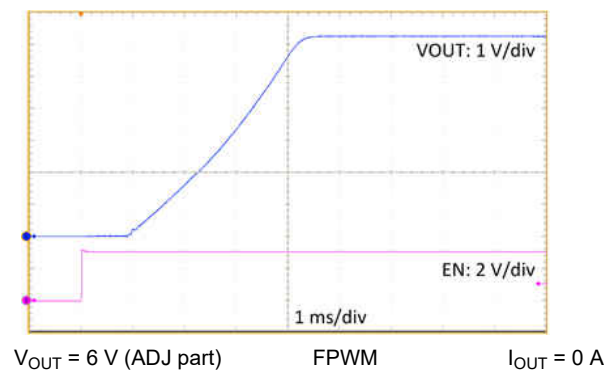
Figure 9-36. Start-up Waveform
