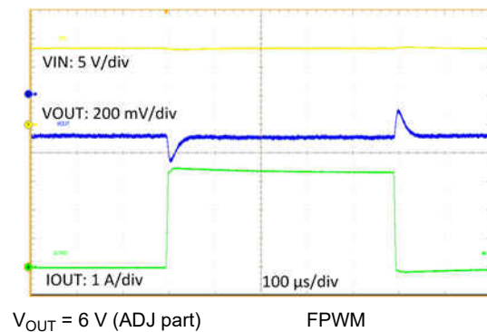
Figure 9-38. Load Transient
