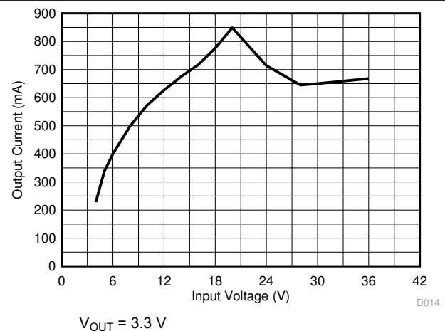
9-24. Load Current for PFM-to-PWM Transition
