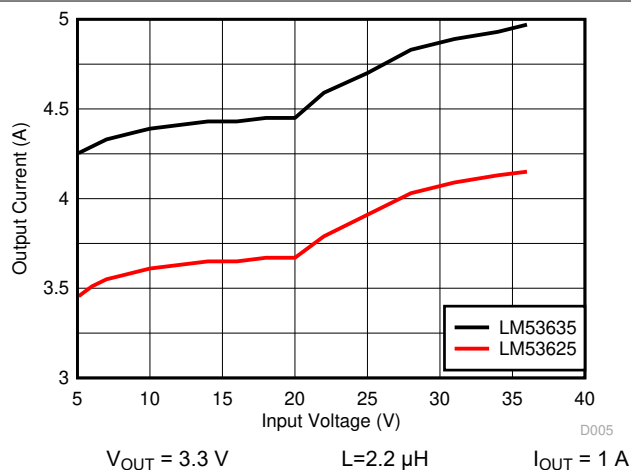
Figure 9-29. Output Current Level for Overcurrent Protection Trip
