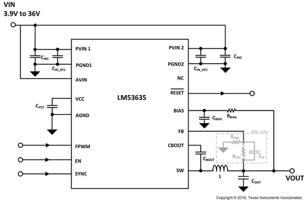
図 9-1. General Application Circuit
