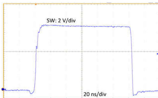
FIG 8-1. Switch Node Waveform ( V_{IN}=13.5V , I_{OUT}=3.5A )
