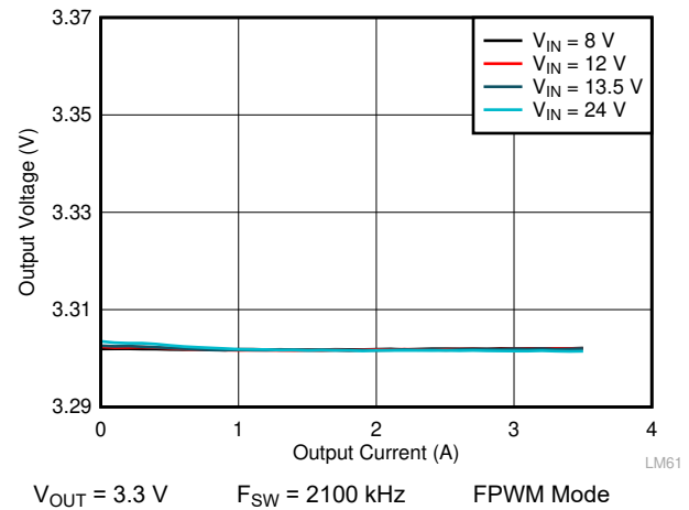
图 9-12. LM61435-Q1 Load and Line Regulation
