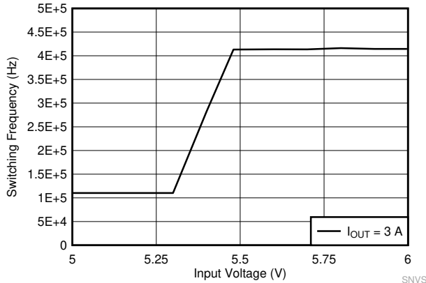
FIG 10-23. LM61440-Q1 Frequency Dropout Curve
