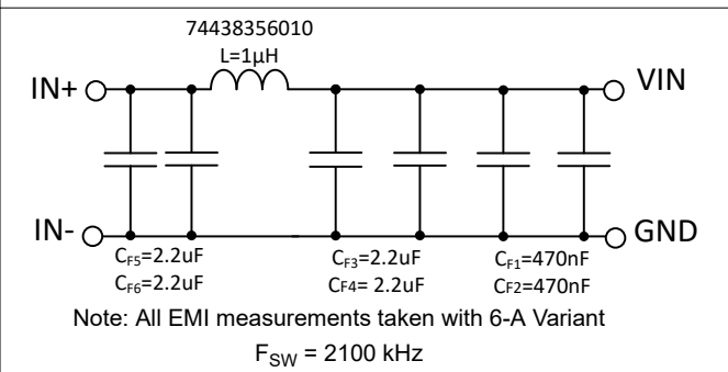
图 10-44. Recommended Input EMI Filter
