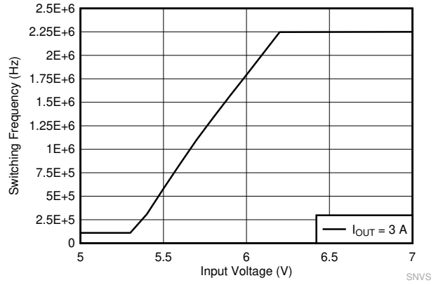
FIG 10-24. LM61440-Q1 Frequency Dropout Curve
