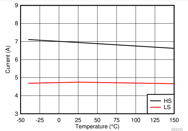
8-4. LM61440-Q1 High-side and Low-side Current Limits
