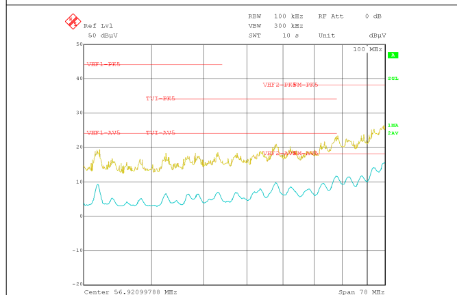
图 10-43. Conducted EMI versus CISPR25 Limits (Yellow: Peak Signal, Blue: Average Signal)
