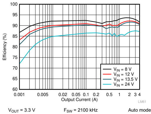
Figure 10-5. LM62440-Q1 Efficiency
