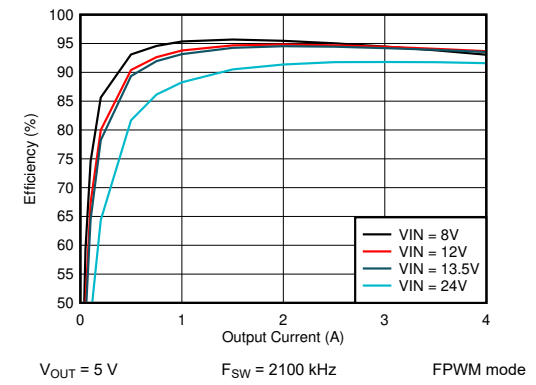
Figure 10-8. LM62440-Q1 Efficiency
