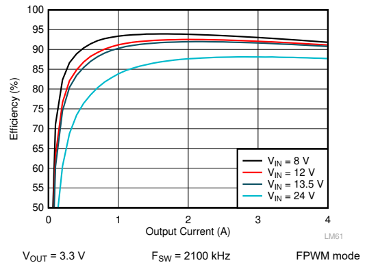
Figure 10-6. LM62440-Q1 Efficiency
