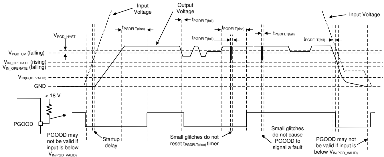
図 9-13. PGOOD Timing Diagram (Excludes OV Events)
