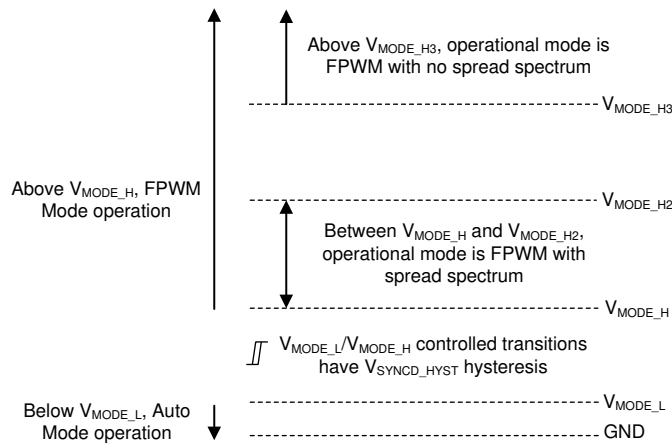
図 9-2. Level-Dependent Mode Selection Settings
