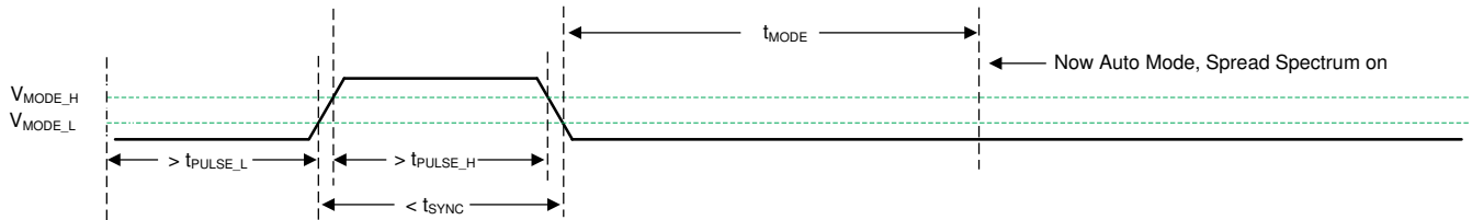
9-10. Transition from SYNC Mode to Auto Mode
