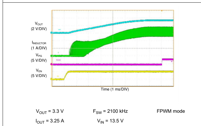
10-19. LM62440-Q1 Start-up with 3.25-A
