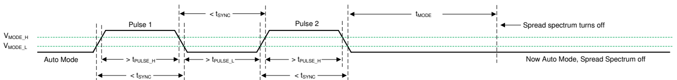
Figure 9-7. Spread Spectrum Disabled in Auto Mode
