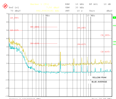
伝導 EMI : V OUT = 5V、f SW = 2100kHz
