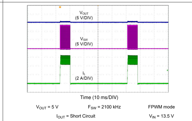
10-22. LM62440-Q1 Short Circuit Performance
