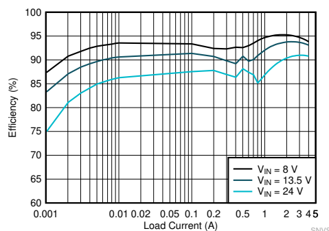
効率 : V OUT = 5V、f SW = 2200kHz
