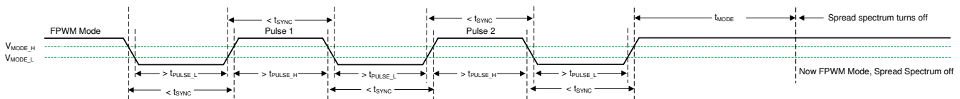
Figure 9-6. Spread Spectrum Disabled in FPWM Mode
