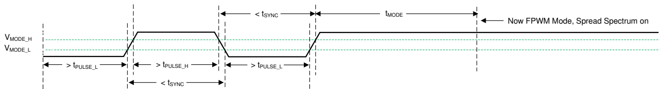
9-11. Transition from SYNC Mode to FPWM Mode
