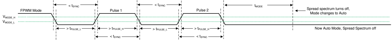
9-8. Spread Spectrum Disabled in Transition from FPWM Mode to Auto Mode
