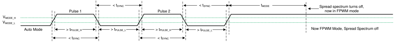
9-9. Spread Spectrum Disabled in Transition from Auto Mode to FPWM Mode
