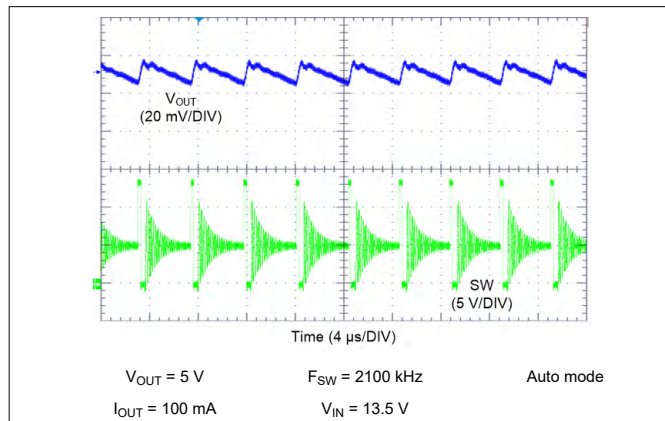
10-17. LM62440-Q1 Switching Waveform and V_{OUT} Ripple
