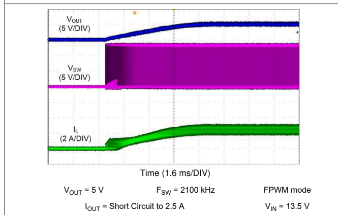
10-21. LM62440-Q1 Short Circuit Recovery
