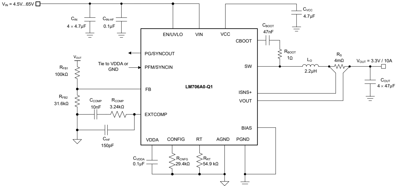
7-23. Application Circuit 2 With LM706A0-Q1 Buck Regulator at 400kHz
