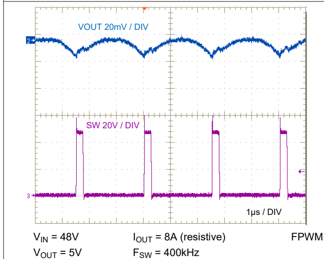
图 7-15. Full Load Switching
