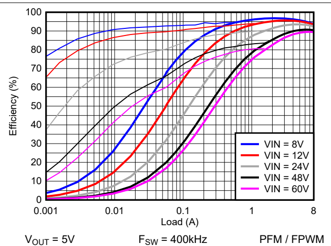
图 7-14. Efficiency versus I_{OUT} , Log Scale
