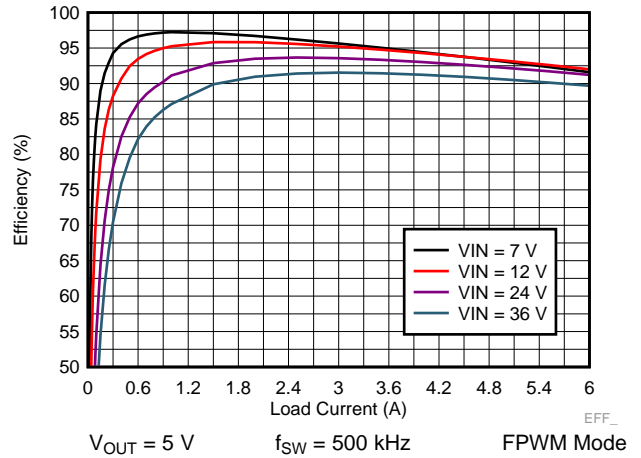
图 34. LM73606 Efficiency
