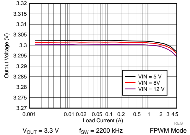
图 46. LM73605 Load and Line Regulation
