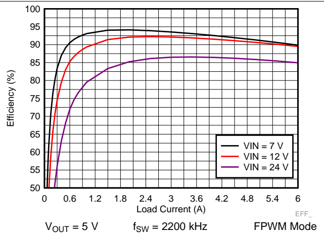
图 38. LM73606 Efficiency
