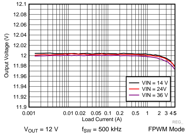
图 50. LM73605 Load and Line Regulation
