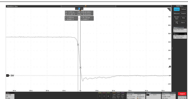
図 8-4. SW Node Behavior Showing the Fall Time for a Buck Converter
