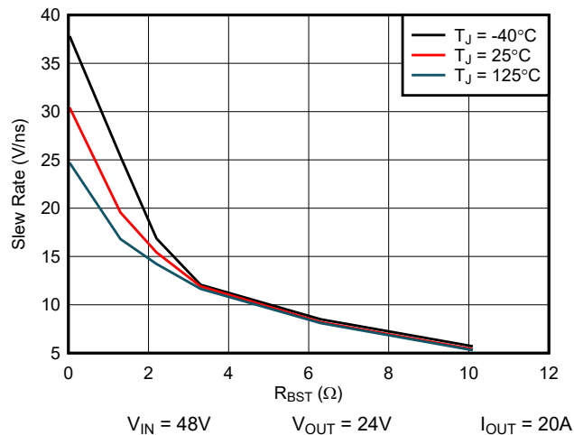
図 5-7. Slew Rate Control for a Buck Converter Using R_{BST}
