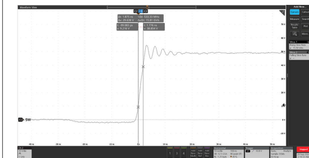
図 8-5. SW Node Behavior Showing the Rise Time for a Buck Converter with HB-HS supplied externally and R_{BST}=1.3\ \Omega
