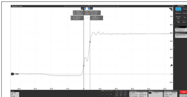
図 8-3. SW Node Behavior Showing the Dead Time and Rise Time for a Buck Converter with R_{BST}=1.3\ \Omega
