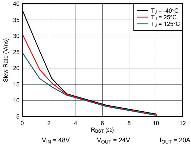
5-7. Slew Rate Control for a Buck Converter Using R_{BST}
