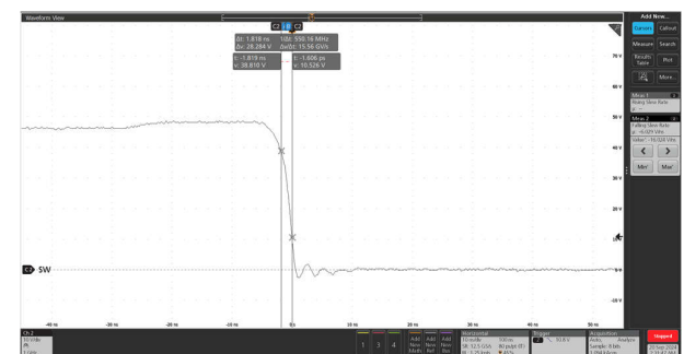
図 8-6. SW Node Behavior Showing the Fall Time for a Boost Converter R_{VCC}=1.3\ \Omega
