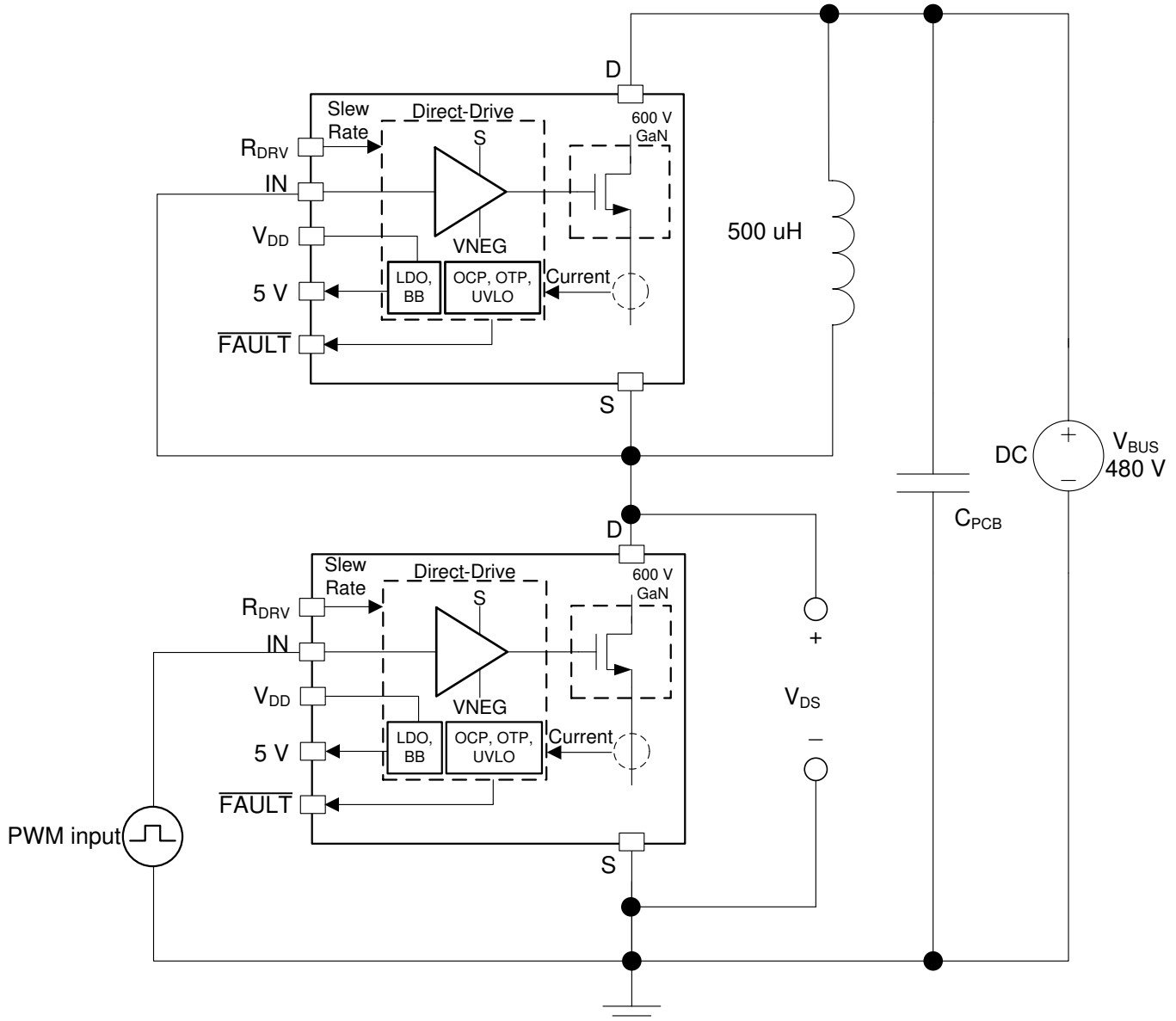
1. Circuit Used to Determine Switching Parameters
