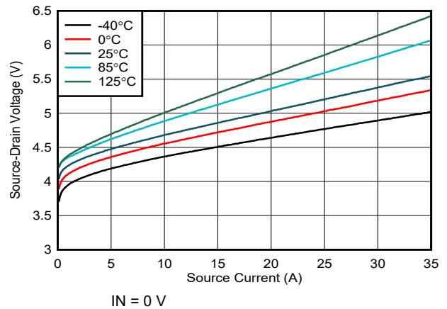
図 5-6. Off-State Source-Drain Voltage vs Source Current
