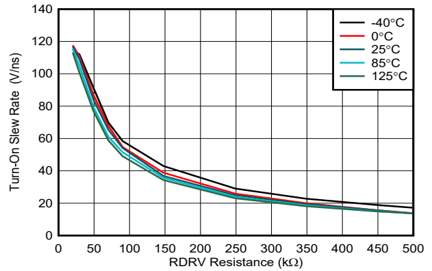
図 5-4. Turn-On Slew Rate vs Drive-Strength Resistance
