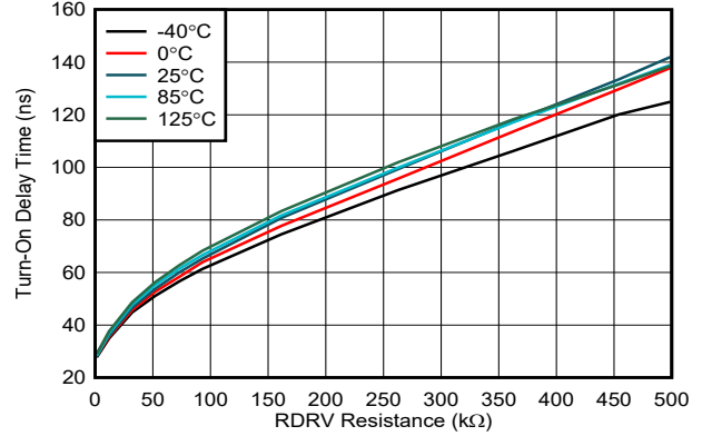
図 5-2. Turn-On Delay Time vs Drive-Strength Resistance
