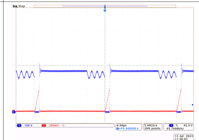
図 8-5. V_{IN} = 230VAC V_{OUT} = 5V I_{OUT} = 3A
