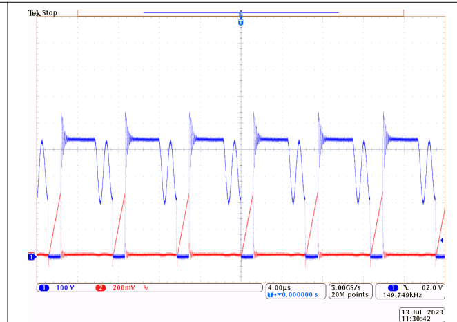
図 8-3. V_{IN} = 230VAC V_{OUT} = 20V I_{OUT} = 3.25A
