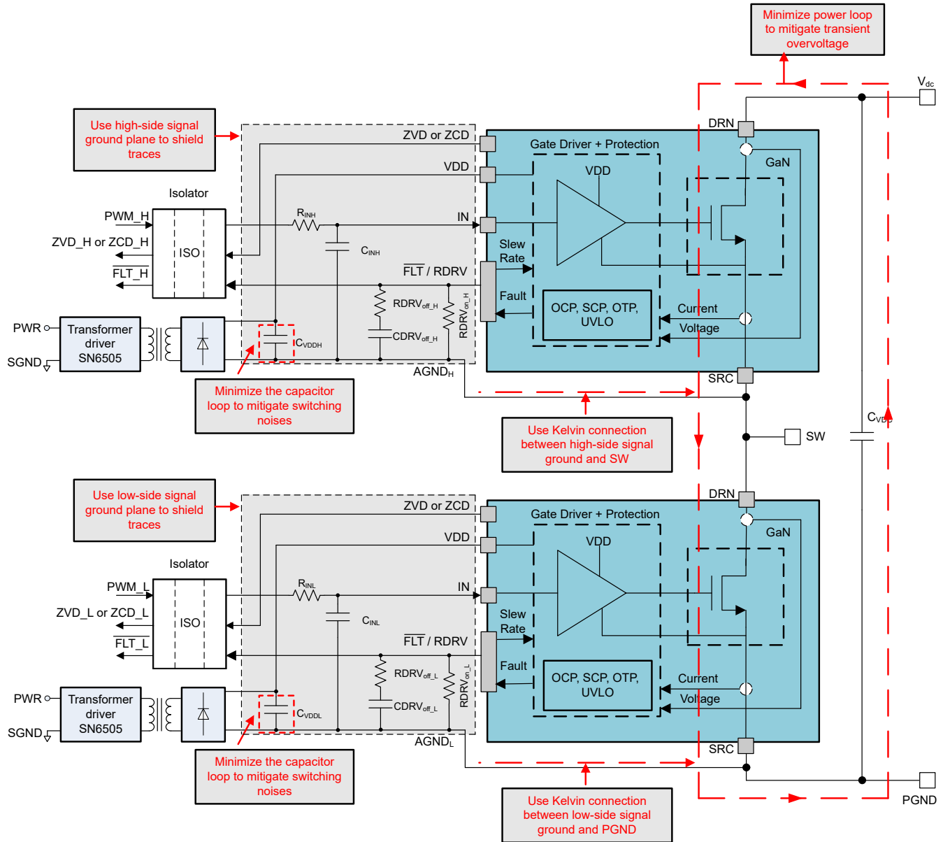
図 9-11. LMG3656R070 or LMG3657R070 Typical Schematic With Layout Considerations
