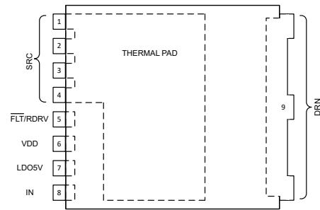
图 5-2. LMG3651R070, TOLL Package (Top View)
