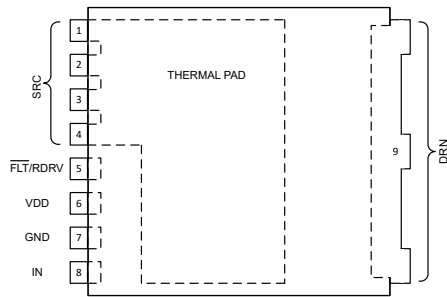
图 5-1. LMG3650R070, TOLL Package (Top View)
