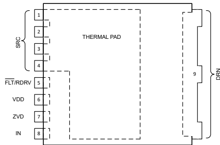
图 5-3. LMG3656R070, TOLL Package (Top View)
