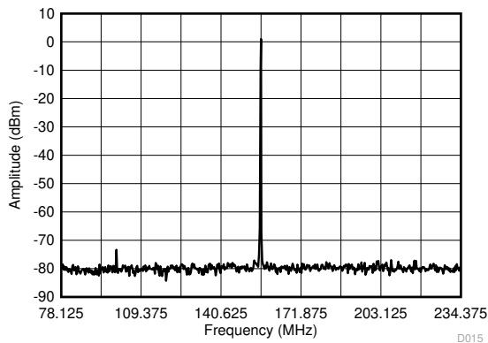
図 6-13. 156.25 ± 78.125-MHz HCSL Output Spectrum With PLL Bandwidth at 1 MHz, Integer N PLL, 50-MHz Crystal Input, 5-GHz VCO Frequency, Post Divider = 8, Output Divider = 4
