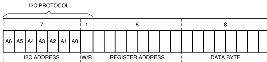
8-32. I 2 C Register Structure
