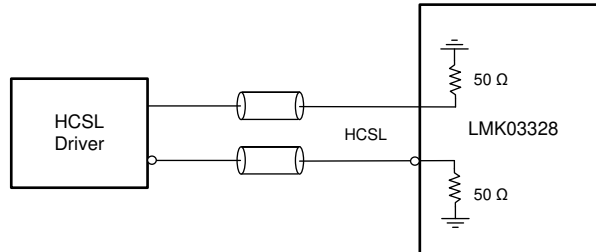
8-11. DC-Coupling LMK03328 Inputs With HCSL Signal
