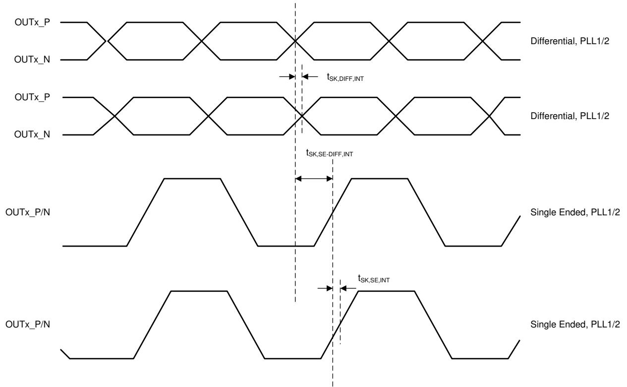
図 7-17. Differential and Single-Ended Output Skew
