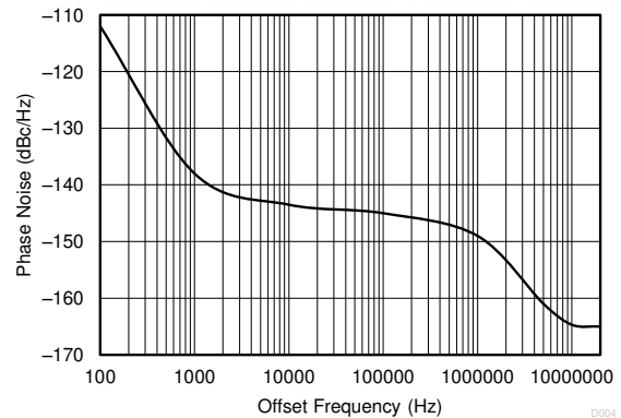
6-2. Closed-Loop Phase Noise of AC-LVPECL Outputs at 156.25 MHz With PLL Bandwidth at 1 MHz, Integer N PLL, 50-MHz Crystal Input, 5-GHz VCO Frequency, Post Divider = 8, Output Divider = 4
