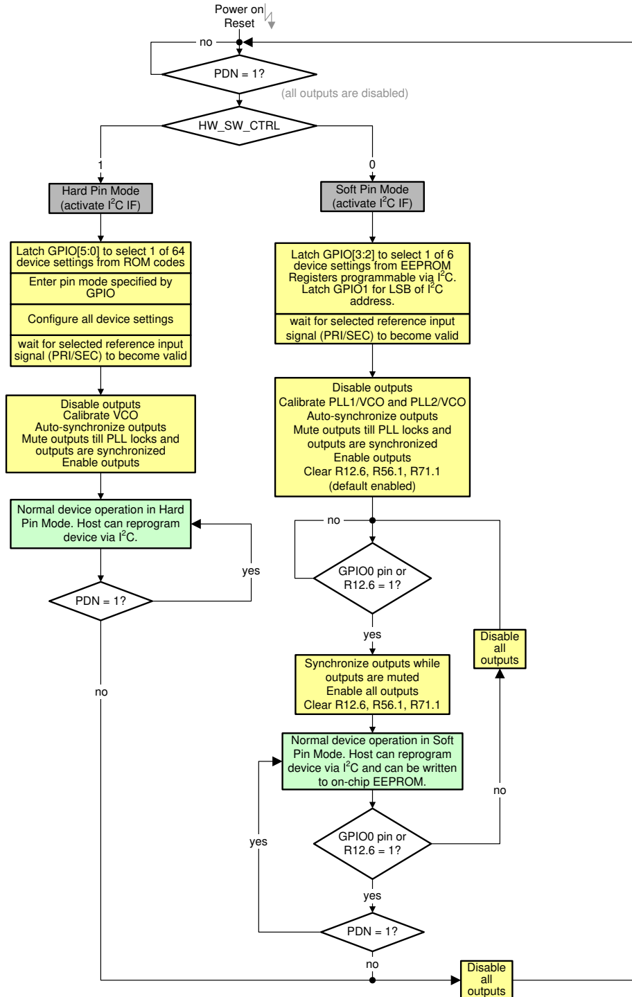
10-9. Flow Chart for Device Power Up and Configuration
