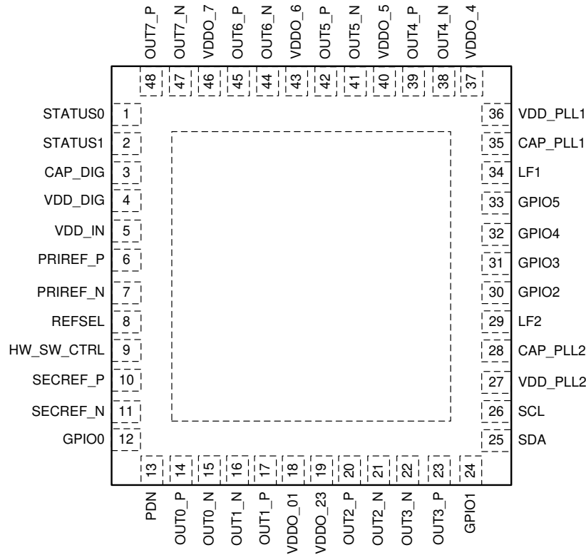
図 5-1. RHS Package 48-Pin QFN Top View
