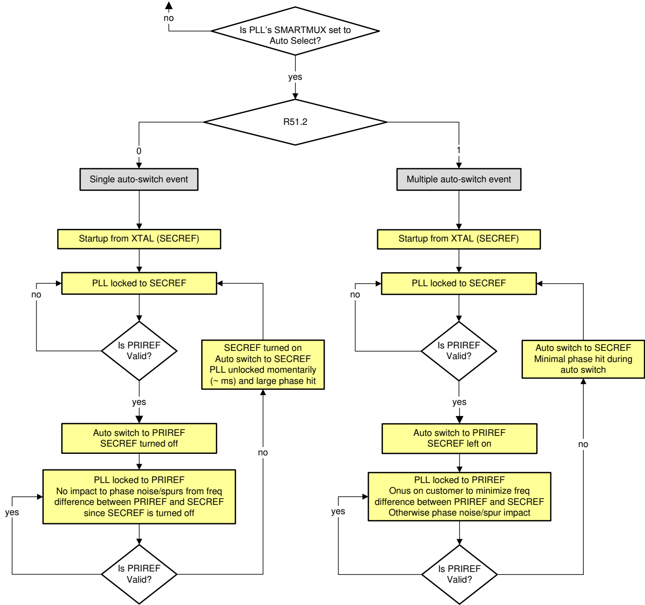
8-4. Flowchart Describing Events When R51.2 is Set to 0 or 1
