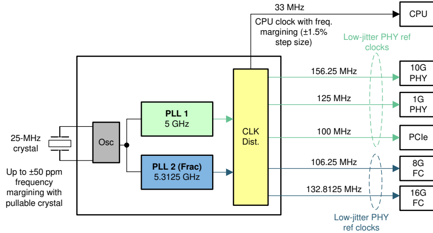
図 10-7. Storage Area Network With Fibre Channel Over Ethernet (FCoE)
