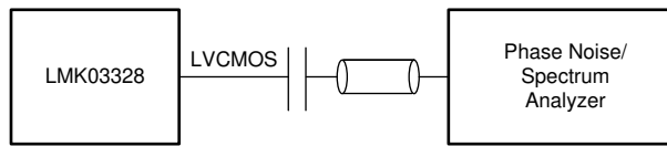
☒ 7-2. LVC MOS Output AC Configuration During Device Test
