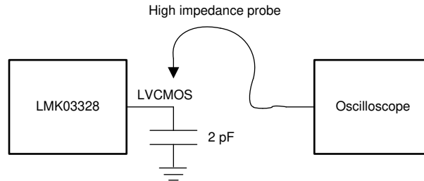
7-1. LVC MOS Output DC Configuration During Device Test
