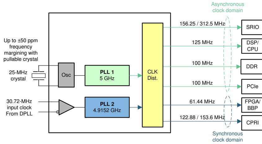
10-6. Wireless Baseband Processing Unit
