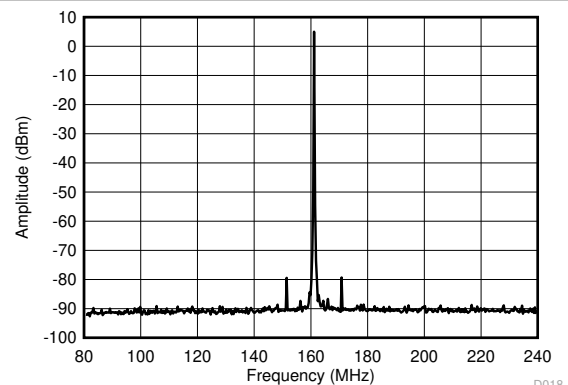
図 6-16. 161.1328125 ± 80.56640625-MHz AC-CML Output Spectrum With PLL Bandwidth at 400 kHz, Fractional N PLL, 50-MHz Crystal Input, 5.15625-GHz VCO Frequency, Post Divider = 8, Output Divider = 4
