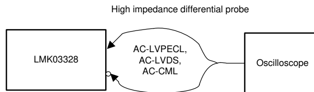
7-3. AC-LVPECL, AC-LVDS, AC-CML Output DC Configuration During Device Test
