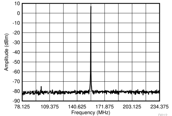
6-10. 156.25 ± 78.125-MHz AC-LVPECL Output Spectrum With PLL Bandwidth at 1 MHz, Integer N PLL, 50-MHz Crystal Input, 5-GHz VCO Frequency, Post Divider = 8, Output Divider = 4
