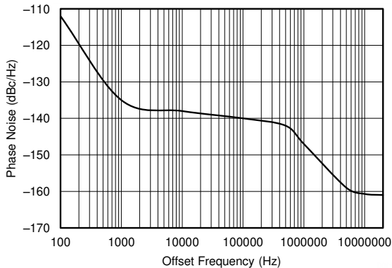
6-9. Closed-Loop Phase Noise of HCSL Outputs at 161.1328125 MHz With PLL Bandwidth at 400 kHz, Fractional N PLL, 50-MHz Crystal Input, 5-GHz VCO Frequency, Post Divider = 8, Output Divider = 4
