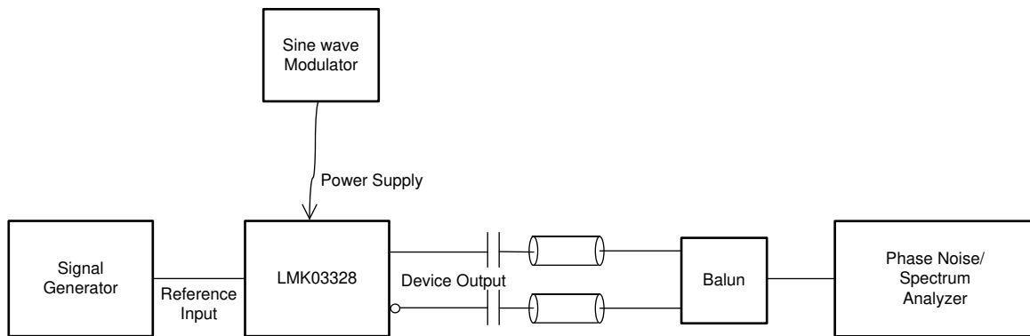
7-14. PSNR Test Setup
