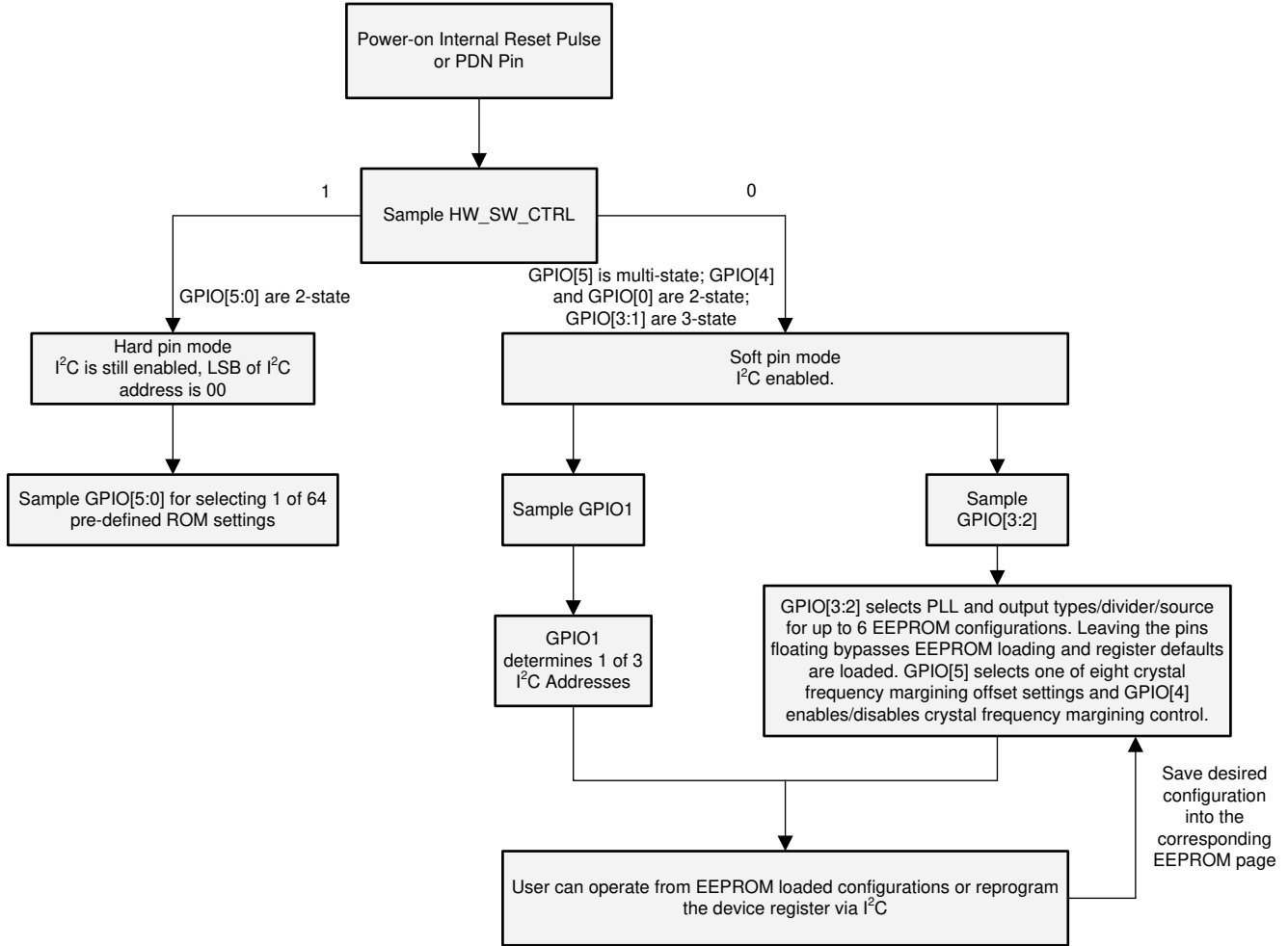
図 8-1. LMK03328 Simplified Programming Flow
