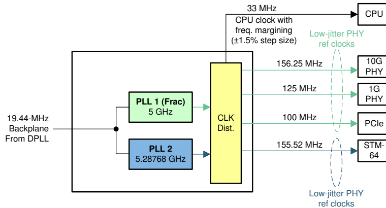
図 10-8. Carrier Ethernet Line Card
