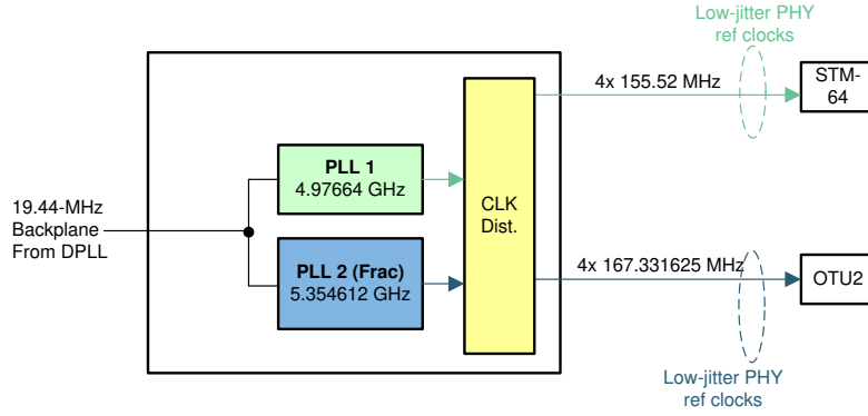
10-5. Optical Transport Network Line Card With FEC (255/237)
