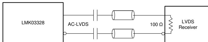
☒ 8-26. Interfacing the LMK03328 AC-LVDS Output With LVDS Receiver
