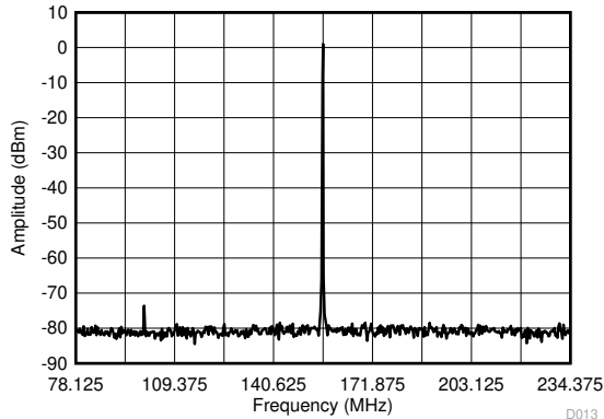
図 6-11. 156.25 ± 78.125-MHz AC-LVDS Output Spectrum With PLL Bandwidth at 1 MHz, Integer N PLL, 50-MHz Crystal Input, 5-GHz VCO Frequency, Post Divider = 8, Output Divider = 4
