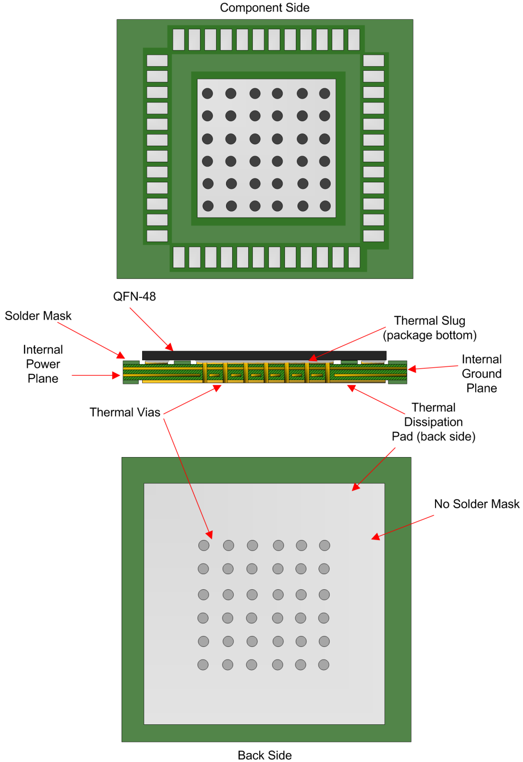
図 10-13. 4-Layer PCB Thermal Layout Example for LMK03328 (8+ Layers Recommended)
