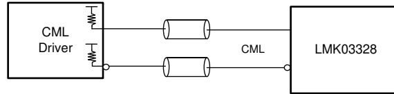
8-10. DC-Coupling LMK03328 Inputs With CML Signal
