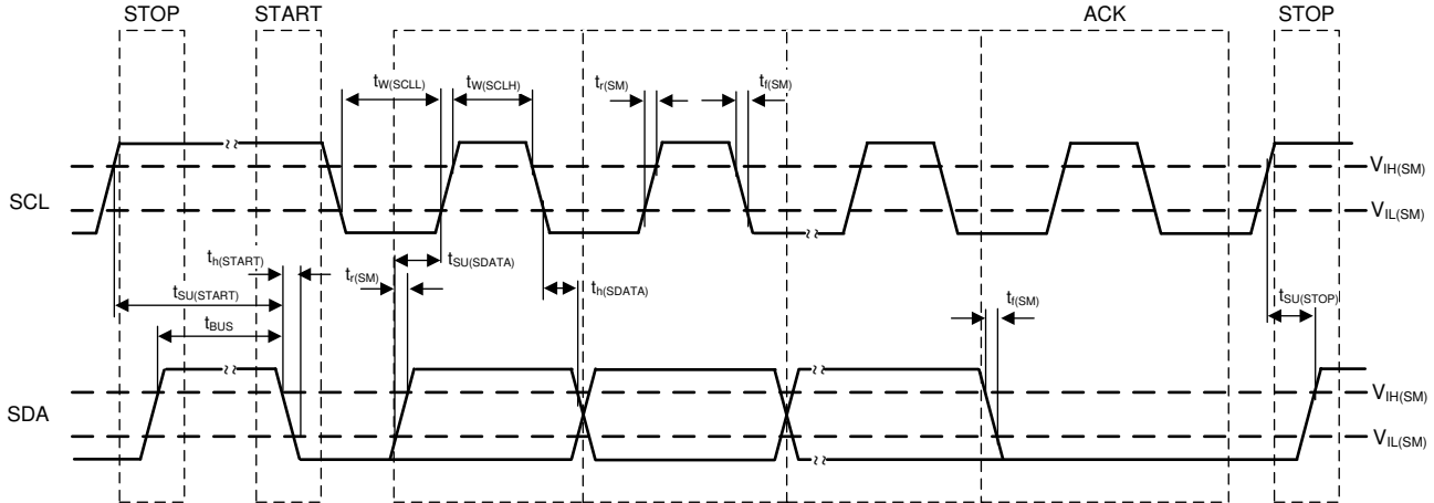
8-31. I 2 C Timing Diagram
