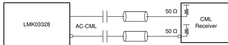
☒ 8-27. Interfacing the LMK03328 AC-CML Output With CML Receiver
