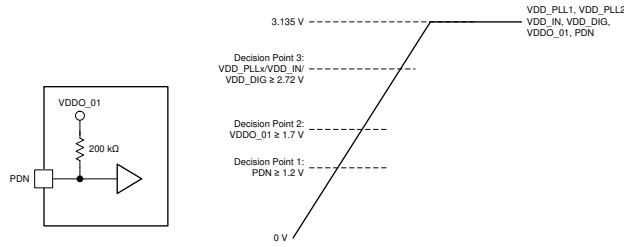
図 10-10. Recommendations for Power Up From Single-Supply Rail
