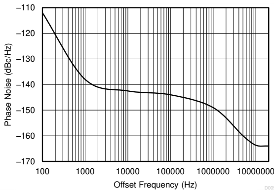
6-3. Closed-Loop Phase Noise of AC-LVDS Outputs at 156.25 MHz With PLL Bandwidth at 1 MHz, Integer N PLL, 50-MHz Crystal Input, 5-GHz VCO Frequency, Post Divider = 8, Output Divider = 4
