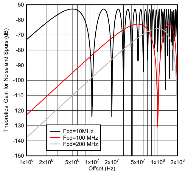
図 8-20. Theoretical Delta Sigma Noise Shaping for 3rd Order Modulator
