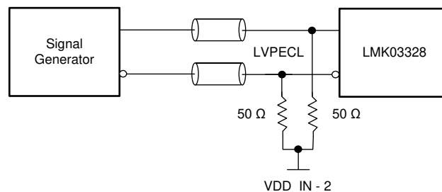
7-10. LVPECL Input DC Configuration During Device Test
