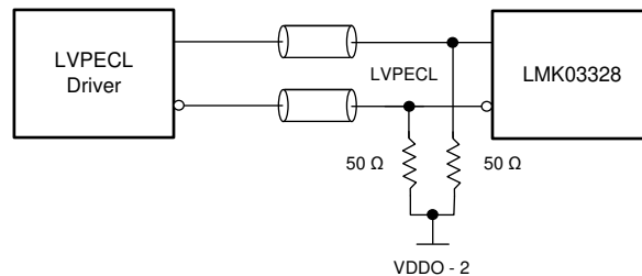
図 8-8. DC-Coupling LMK03328 Inputs With LVPECL Signal
