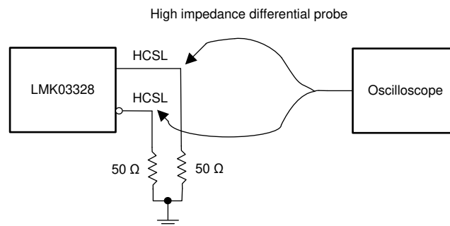
7-4. HC SL Output DC Configuration During Device Test
