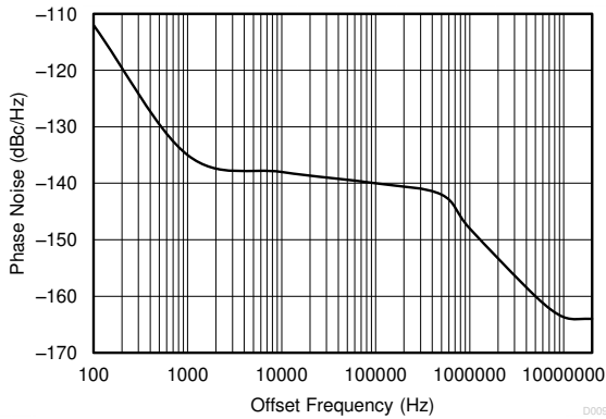
6-7. Closed-Loop Phase Noise of AC-LVDS Outputs at 161.1328125 MHz With PLL Bandwidth at 400 kHz, Fractional N PLL, 50-MHz Crystal Input, 5-GHz VCO Frequency, Post Divider = 8, Output Divider = 4
