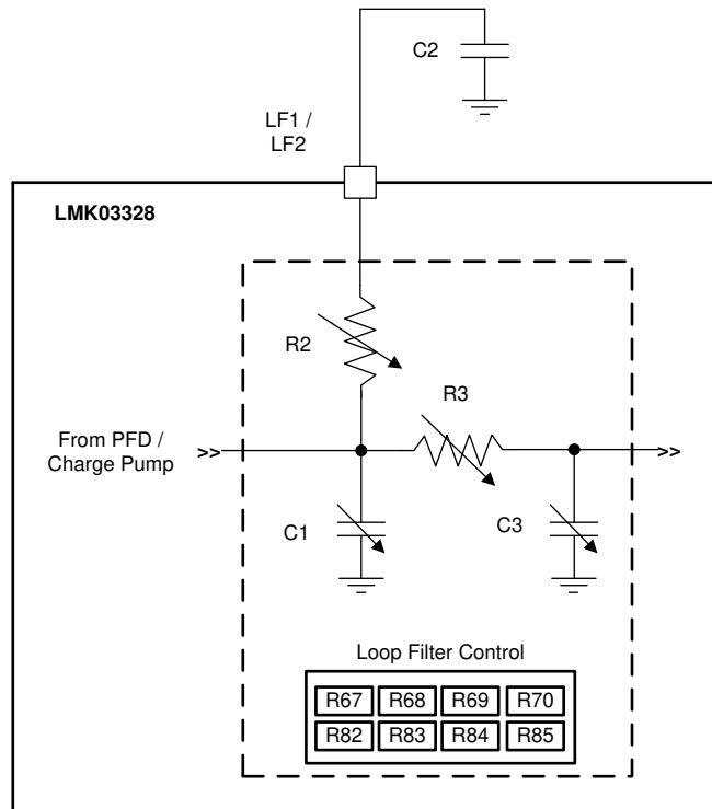
図 8-18. Loop Filter Structure of PLL1 and PLL2
