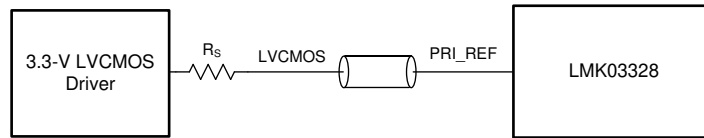
図 8-6. Interfacing LMK03328 Primary Input With 3.3-V LVC MOS Signal
