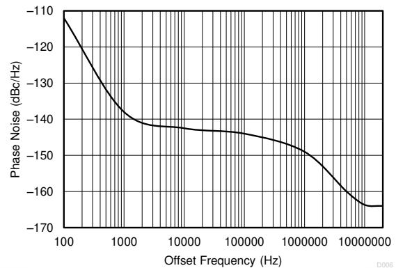
6-4. Closed-Loop Phase Noise of AC-CML Outputs at 156.25 MHz With PLL Bandwidth at 1 MHz, Integer N PLL, 50-MHz Crystal Input, 5-GHz VCO Frequency, Post Divider = 8, Output Divider = 4
