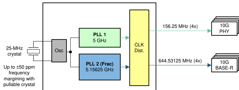
图 10-4. Ethernet Switch With Frac-N PLL for 10GBASE-R (LAN)
