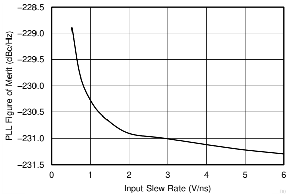
6-1. PLL Figure of Merit (FOM) vs. Slew Rate
