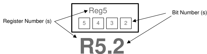
☒ 8-2. LMK03328 Register Reference Format
