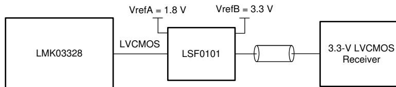
☒ 8-24. Interfacing the LMK03328 1.8-V LVCMOS Output With 3.3-V LVCMOS Receiver
