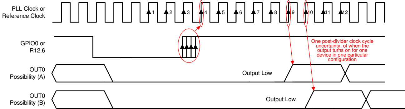
図 8-29. SYNCN to Output Delay Variation
