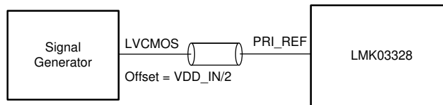
7-7. LVCMOS Primary Input DC Configuration During Device Test
