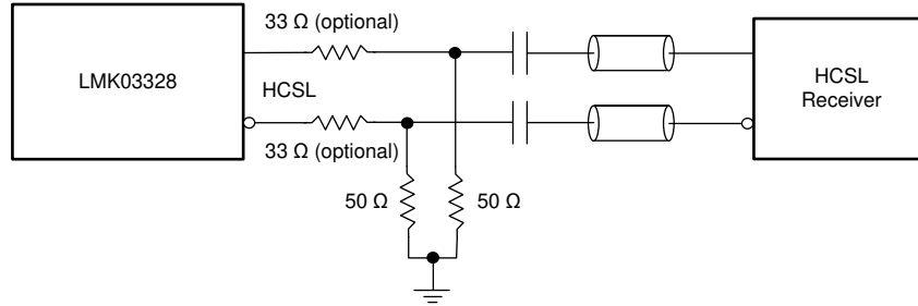
図 8-28. Interfacing the LMK03328 Output With HCSL Receiver
