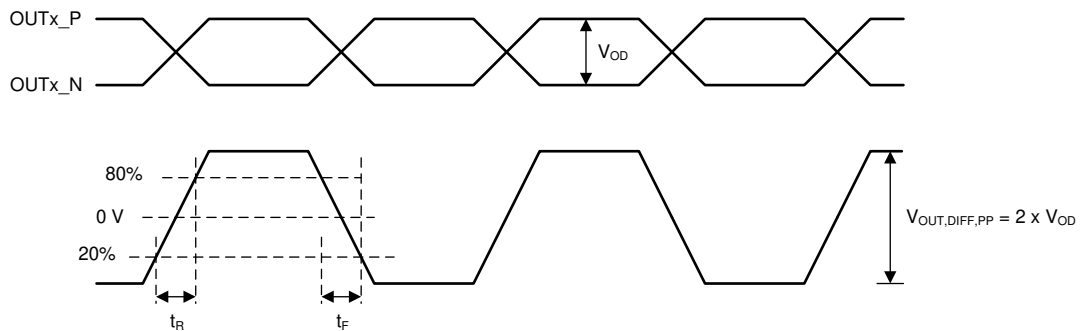
7-15. Differential Output Voltage and Rise/Fall Time
