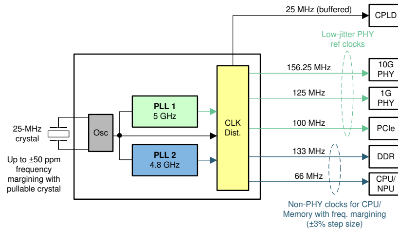
図 10-3. 10-Gb Ethernet Switch/Router Line Card
