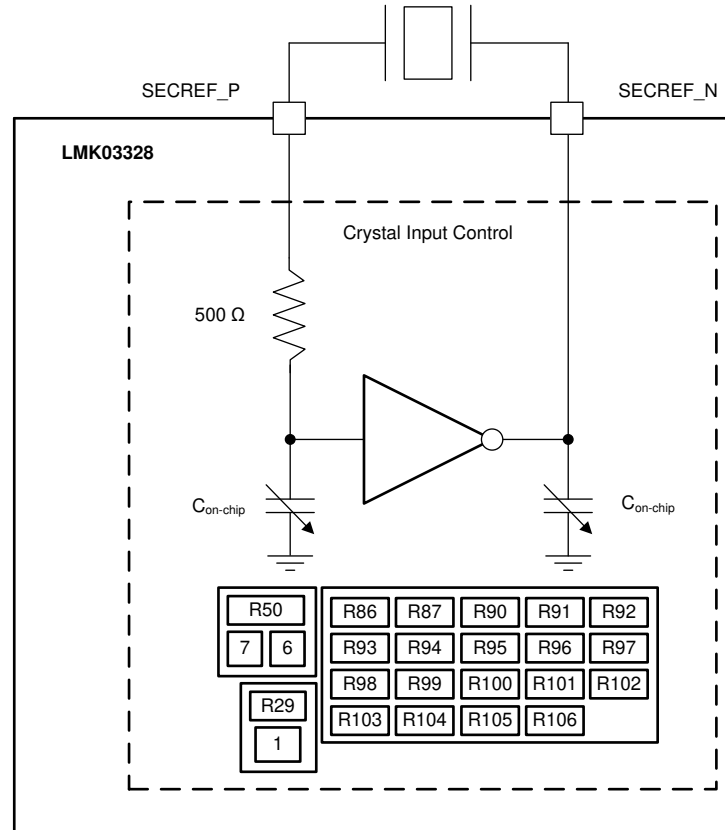
図 8-16. Crystal Input Interface on Secondary Reference
