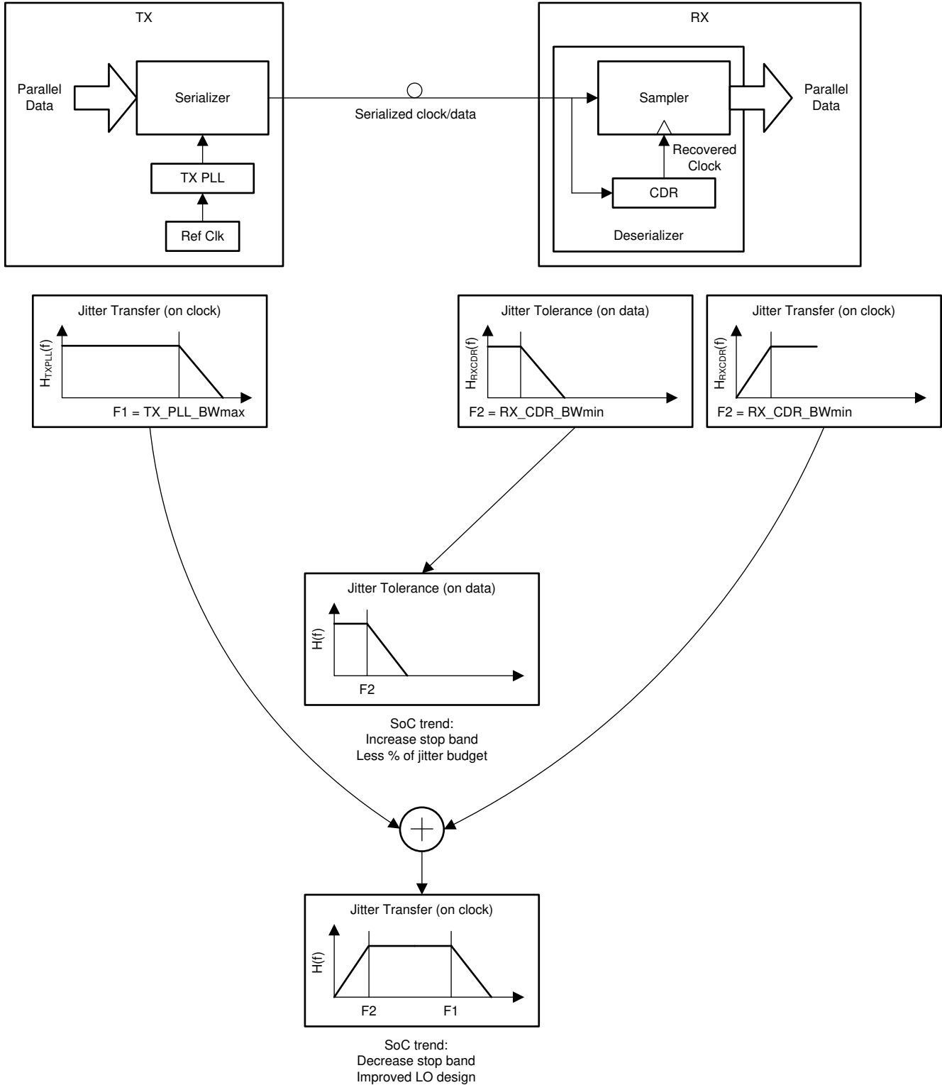
10-1. Dependence of Clock Jitter in Serial Links
