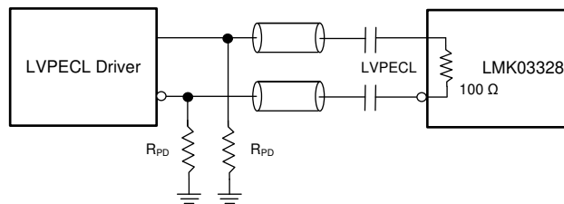
8-12. AC-Coupling LMK03328 Inputs With LVPECL Signal
