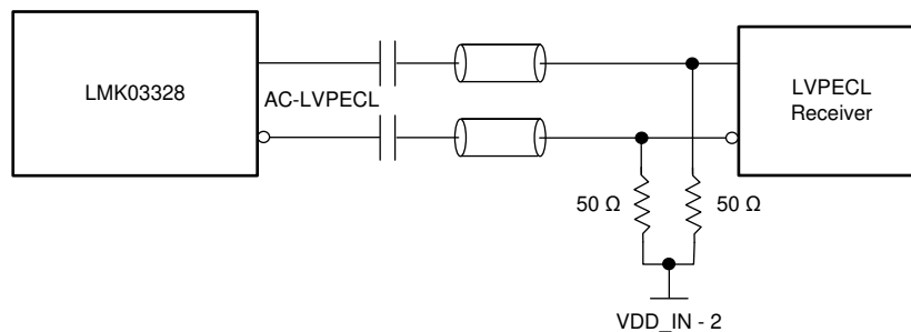
☒ 8-25. Interfacing the LMK03328 AC-LVPECL Output With LVPECL Receiver
