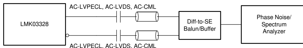
7-5. AC-LVPECL, AC-LVDS, AC-CML Output AC Configuration During Device Test
