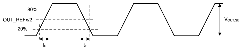
7-16. Single-Ended Output Voltage and Rise/Fall Time
