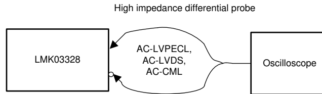
☒ 7-3. AC-LVPECL, AC-LVDS, AC-CML Output DC Configuration During Device Test
