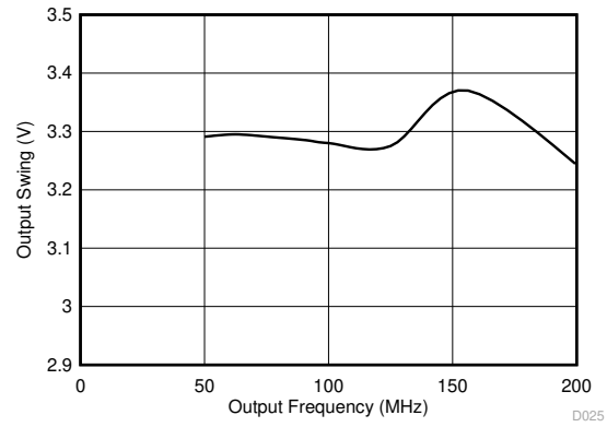
図 6-23. 3.3-V LVCMOS (on STATUS[1:0]) Output Swing vs. Frequency
