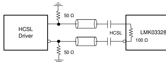
8-15. AC-Coupling LMK03328 Inputs With HCSL Signal
