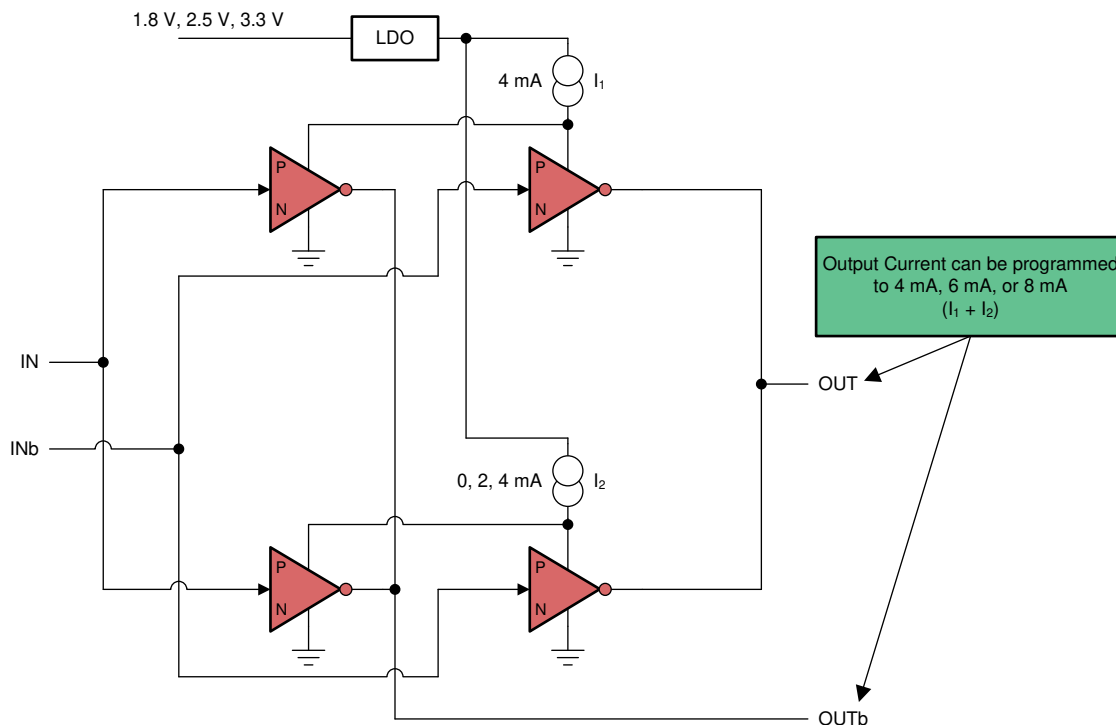
8-22. Structure of AC-LVDS, AC-CML, and AC-LVPECL Output Stage
