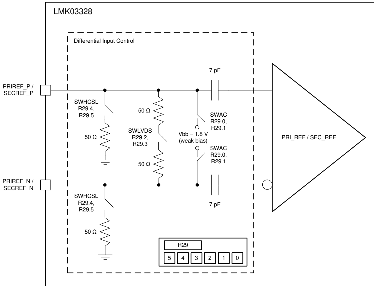
図 8-5. Differential Input Buffer Termination Options on Primary and Secondary Reference
