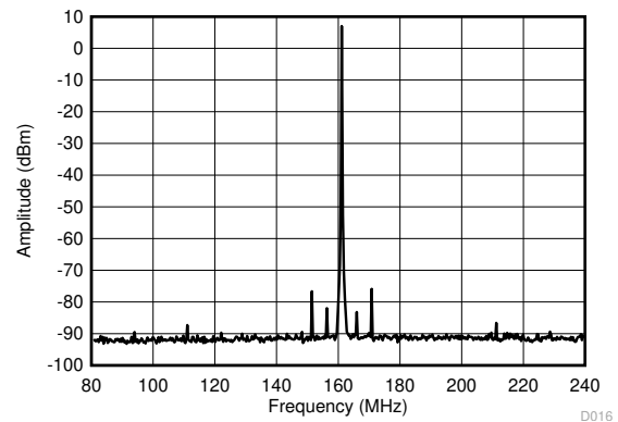
図 6-14. 161.1328125 ± 80.56640625-MHz AC-LVPECL Output Spectrum With PLL Bandwidth at 400 kHz, Fractional N PLL, 50-MHz Crystal Input, 5.15625-GHz VCO Frequency, Post Divider = 8, Output Divider = 4
