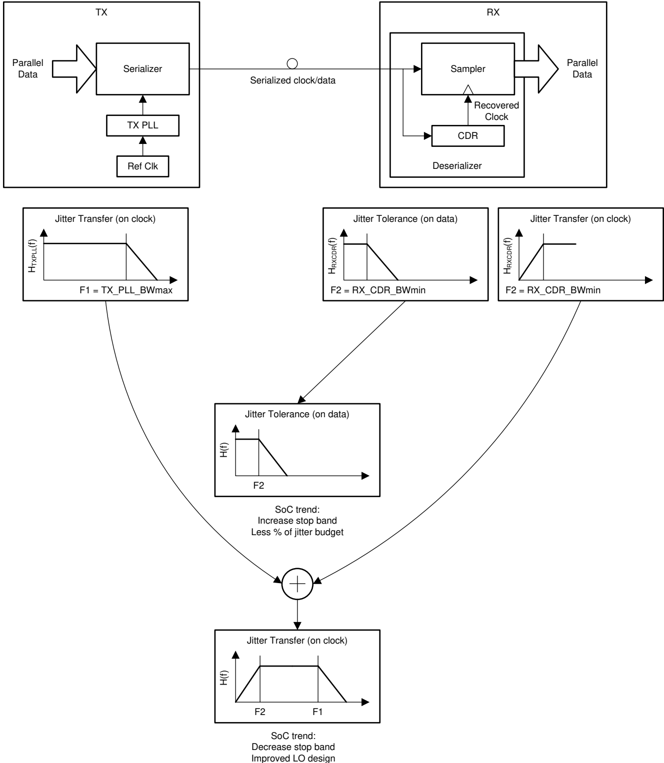
10-1. Dependence of Clock Jitter in Serial Links
