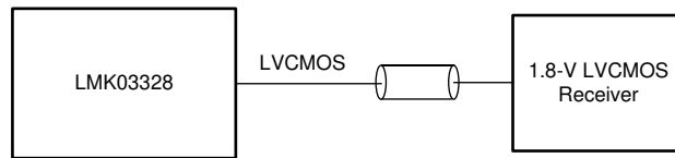
☒ 8-23. Interfacing the LMK03328 1.8-V LVCMOS Output With 1.8-V LVCMOS Receiver
