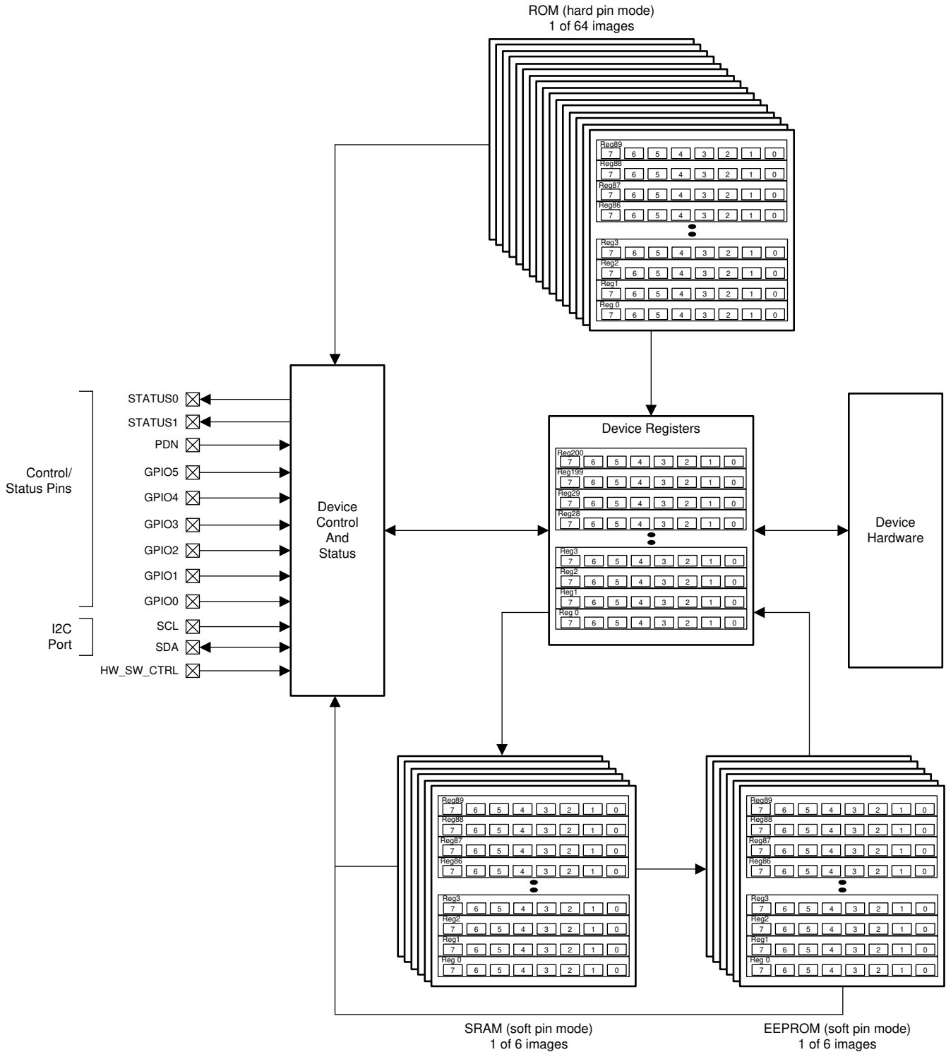
図 8-30. LMK03328 Interface and Control Block
