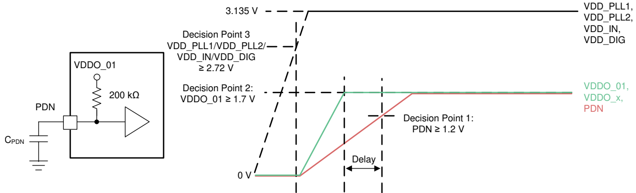
図 10-11. Recommendations for Power Up From Split-Supply Rails
