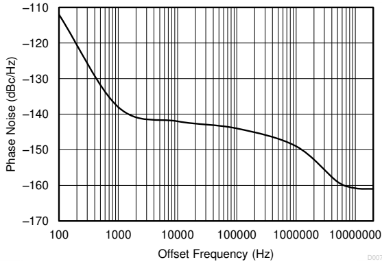
6-5. Closed-Loop Phase Noise of HCSL Outputs at 156.25 MHz With PLL Bandwidth at 1 MHz, Integer N PLL, 50-MHz Crystal Input, 5-GHz VCO Frequency, Post Divider = 8, Output Divider = 4
