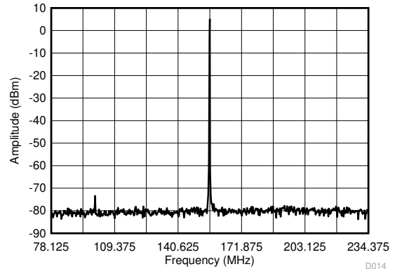
図 6-12. 156.25 ± 78.125-MHz AC-CML Output Spectrum With PLL Bandwidth at 1 MHz, Integer N PLL, 50-MHz Crystal Input, 5-GHz VCO Frequency, Post Divider = 8, Output Divider = 4
