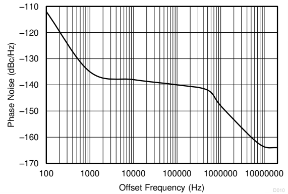
6-8. Closed-Loop Phase Noise of AC-CML Outputs at 161.1328125 MHz With PLL Bandwidth at 400 kHz, Fractional N PLL, 50-MHz Crystal Input, 5-GHz VCO Frequency, Post Divider = 8, Output Divider = 4
