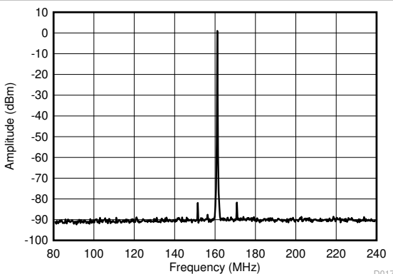
図 6-15. 161.1328125 ± 80.56640625-MHz AC-LVDS Output Spectrum With PLL Bandwidth at 400 kHz, Fractional N PLL, 50-MHz Crystal Input, 5.15625-GHz VCO Frequency, Post Divider = 8, Output Divider = 4
