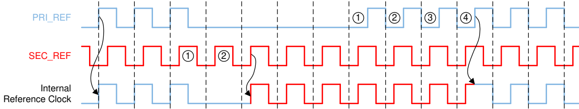
図 8-3. Smart Input MUX Auto Switch Mode Timing Diagram
