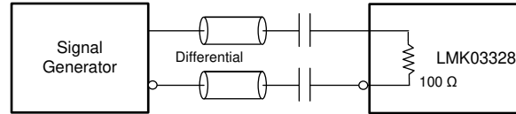
7-12. Differential Input AC Configuration During Device Test
