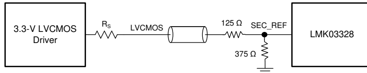
図 8-7. Interfacing LMK03328 Secondary Input With 3.3-V LVC MOS Signal
