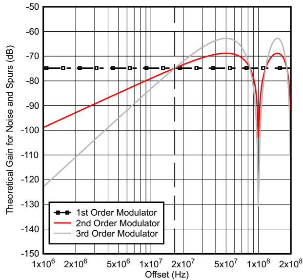
図 8-19. Theoretical Delta Sigma Noise Shaping for a 100-MHz Phase Detector Frequency
