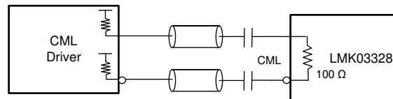
8-14. AC-Coupling LMK03328 Inputs With CML Signal
