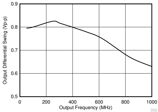
Figure 6-19. AC-LVDS Differential Output Swing vs. Frequency
