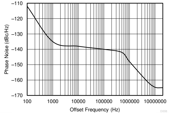
6-6. Closed-Loop Phase Noise of AC-LVPECL Outputs at 161.1328125 MHz With PLL Bandwidth at 400 kHz, Fractional N PLL, 50-MHz Crystal Input, 5.15625-GHz VCO Frequency, Post Divider = 8, Output Divider = 4
