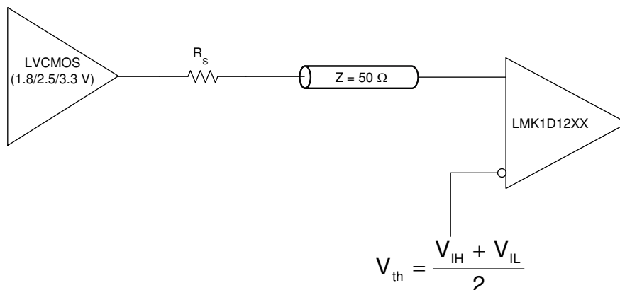
9-6. 1.8-V/2.5-V/3.3-V LVCMOS Clock Driver Connected to LMK1D120x Input
