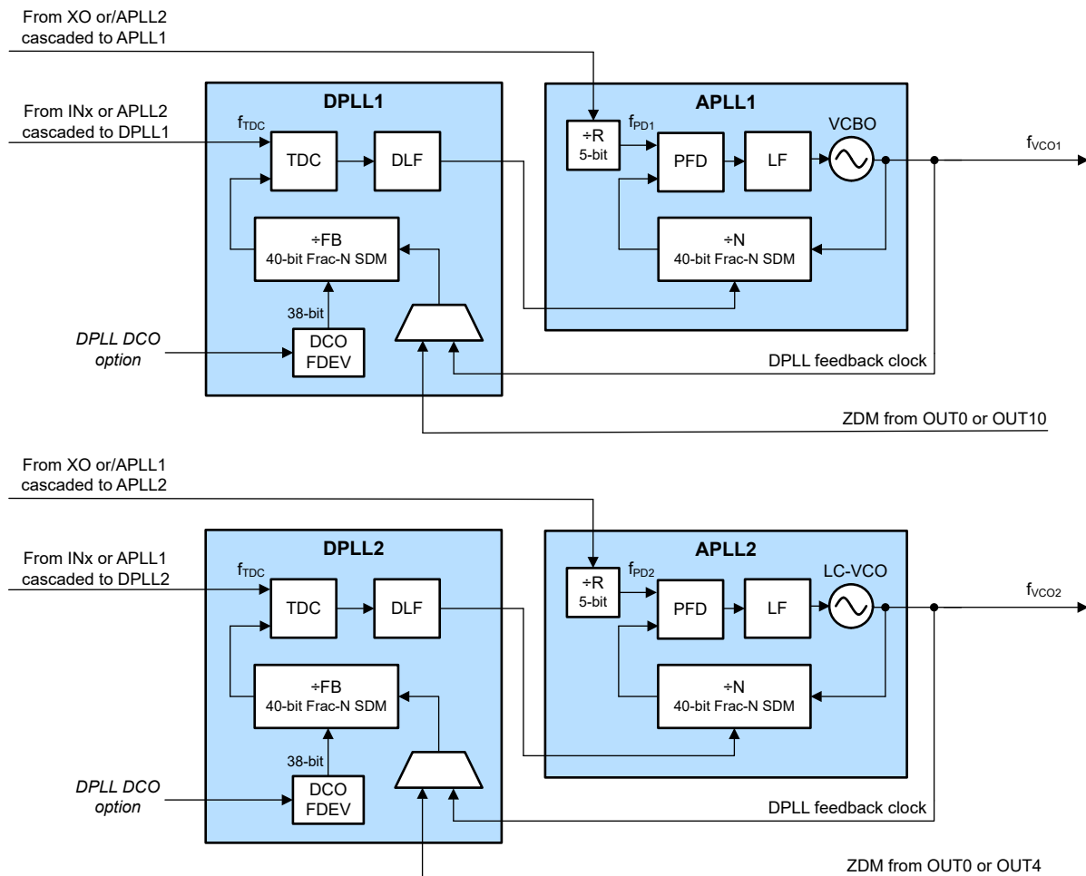
図 7-2. PLL Architecture
