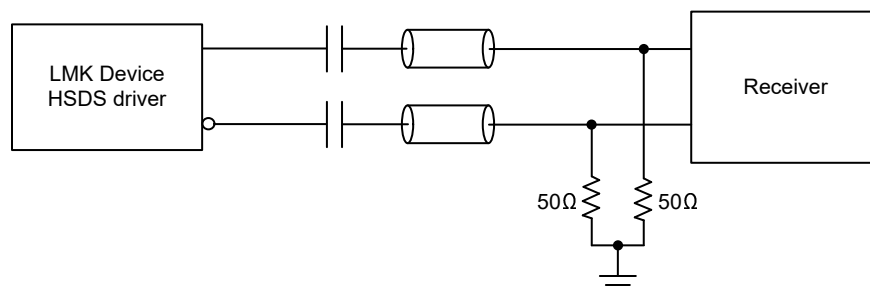
図 7-28. AC-Coupled HSDS Output Termination Method 2
