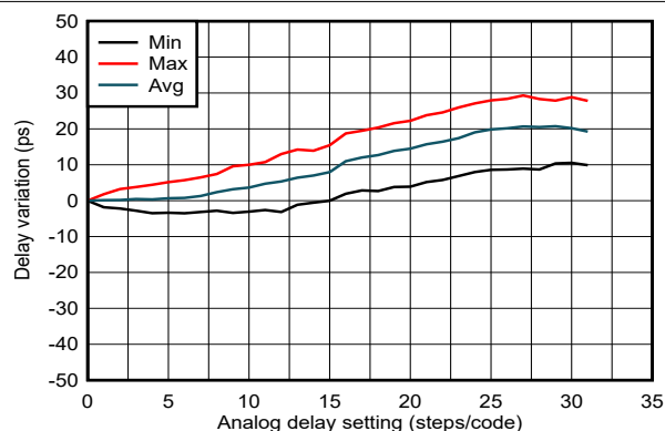
図 5-17. SYSREF/1PPS Delay Linearity vs. Analog Delay Code 2
