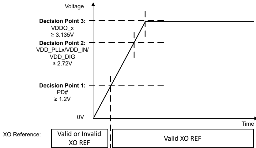
図 8-1. Recommendation for Power Up From a Single-Supply Rail
