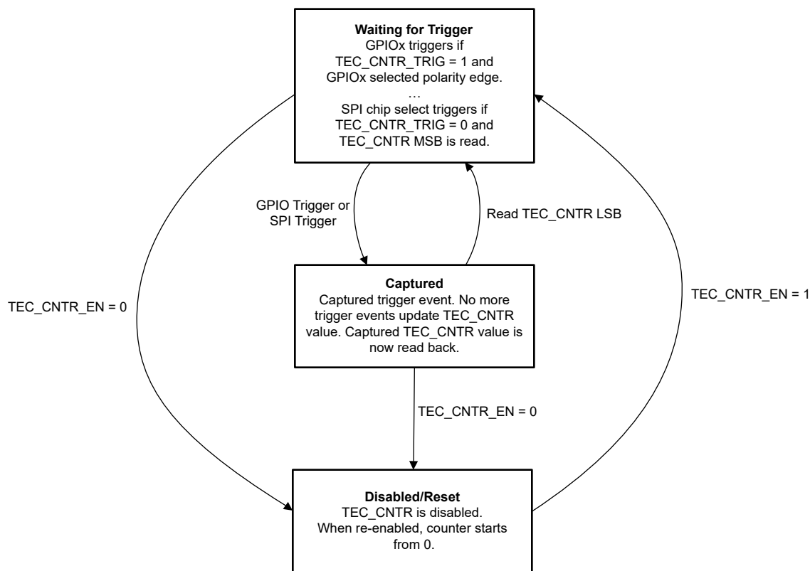
図 7-33. State Diagram of TEC
