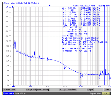
図 5-8. 491.52MHz HSDS Output From APLL1 BAW
