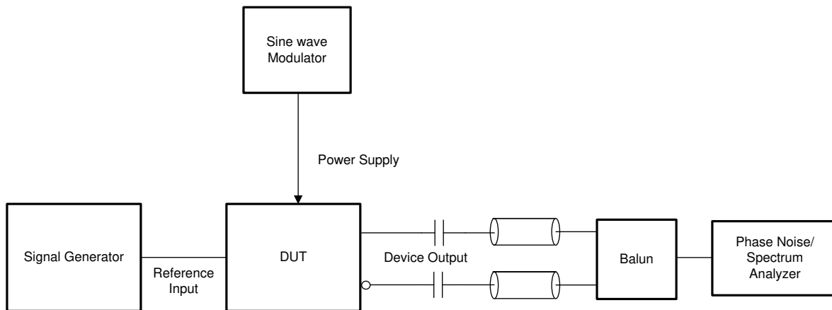
図 6-8. HCSL Output Phase Domain Test Configuration
