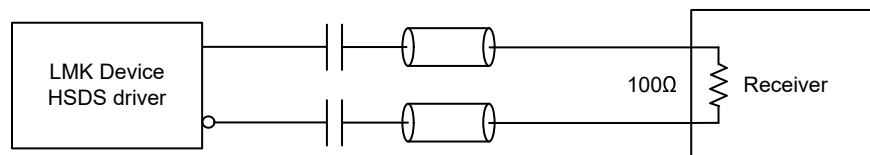
図 7-27. AC-Coupled HSDS Output Termination Method 1
