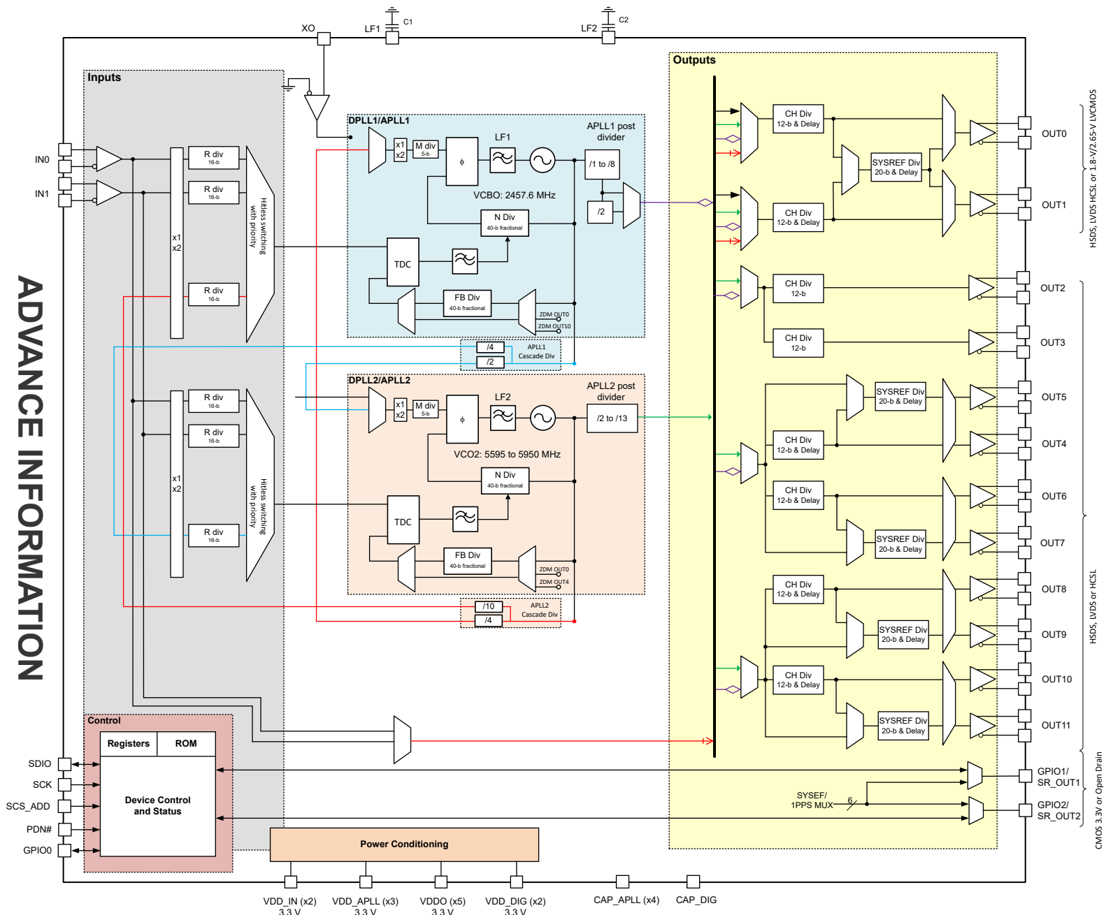
図 7-1. LMK5C22212AS1 Top-Level Block Diagram
