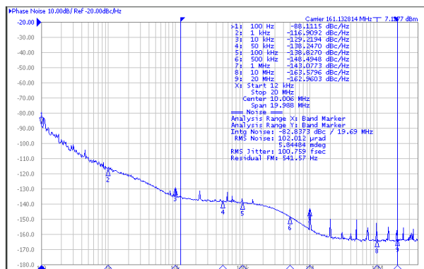
図 5-14. 161.1328125MHz HSDS Output From APLL2
