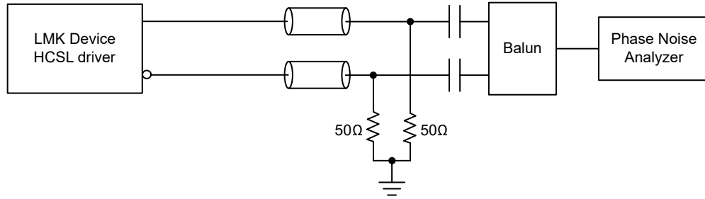
図 6-8. HCSL Output Phase Domain Test Configuration
