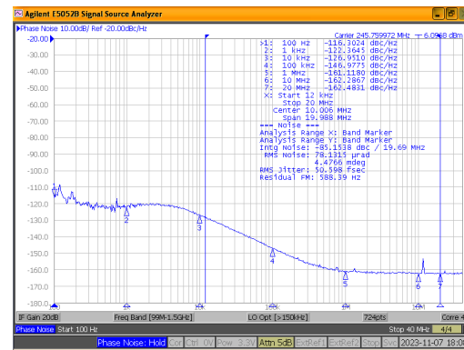
図 5-9. 245.76MHz HSDS Output From APLL1 BAW
