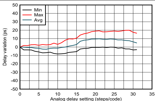
図 5-18. SYSREF/1PPS Delay Linearity vs. Analog Delay Code 3
