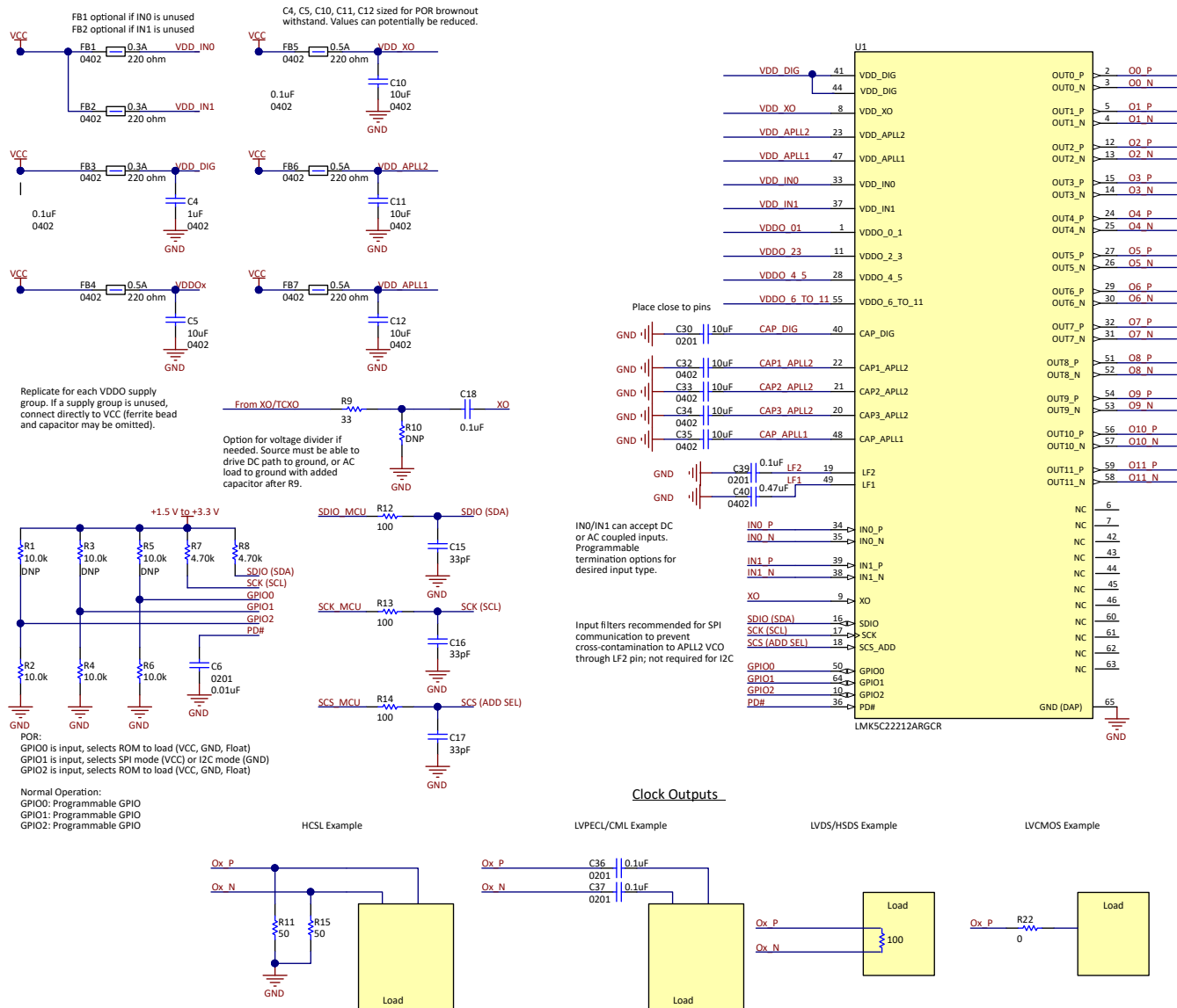
8-3. Reference Schematic Example
