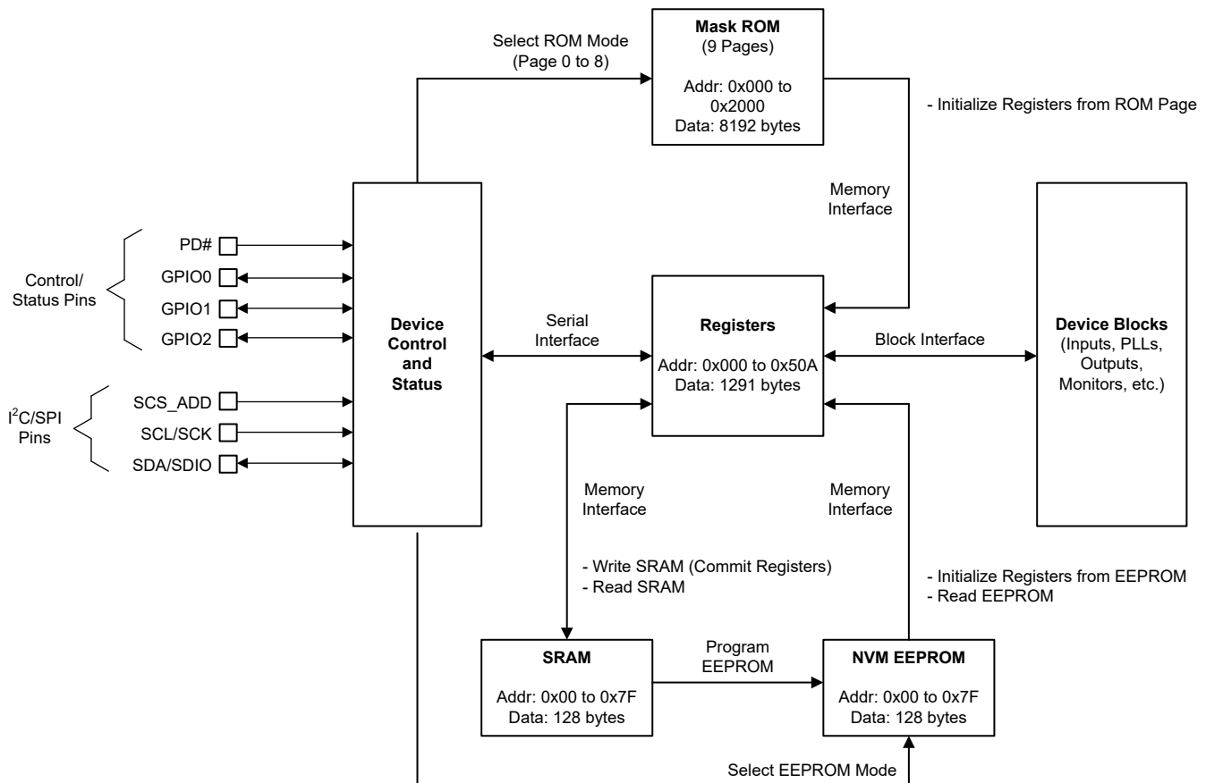
図 7-42. Device Control, Register, and Memory Interfaces
