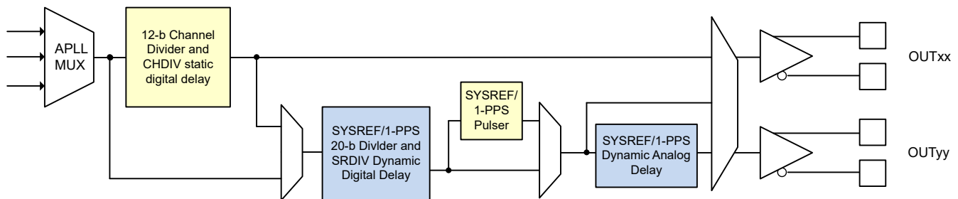
図 7-24. Programmable Static and Dynamic Output Delay
