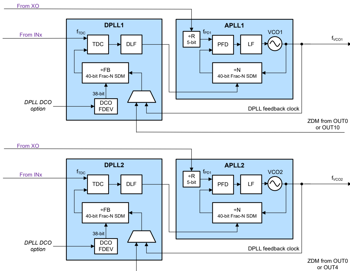
7-3. DPLL Operation
