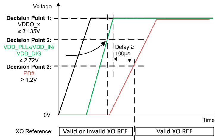
図 8-2. Recommendation for Power Up From Split-Supply Rails
