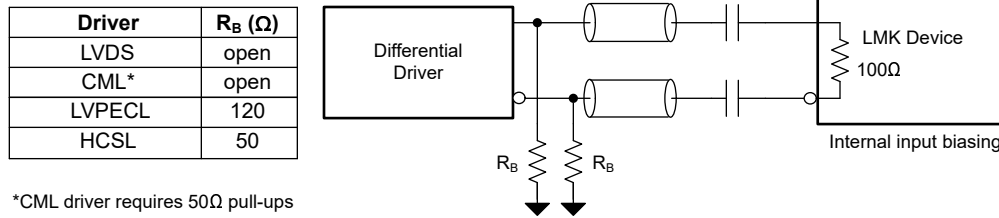
図 7-14. AC-Coupled Differential to Reference (INx)
