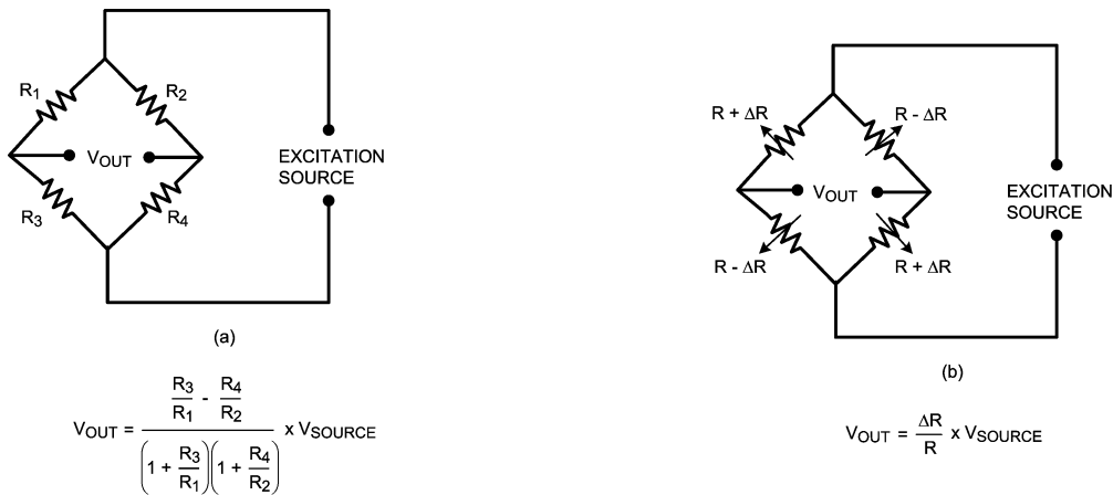
FIGURE 4. Bridge Sensor
