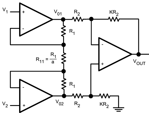
FIGURE 3. Instrumentation Amplifier
