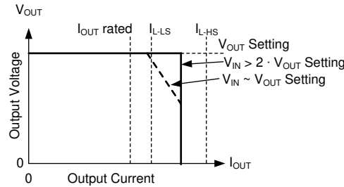
8-14. Output Voltage versus Output Current
