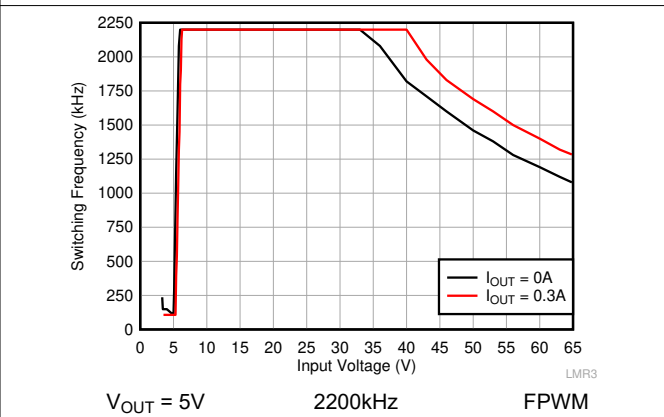
8-19. Switching Frequency over Input Voltage
