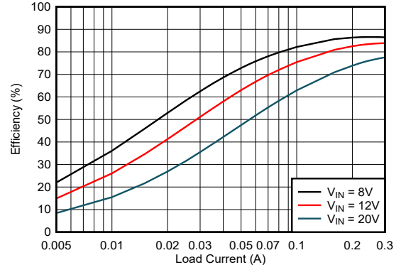
8-11. Efficiency
