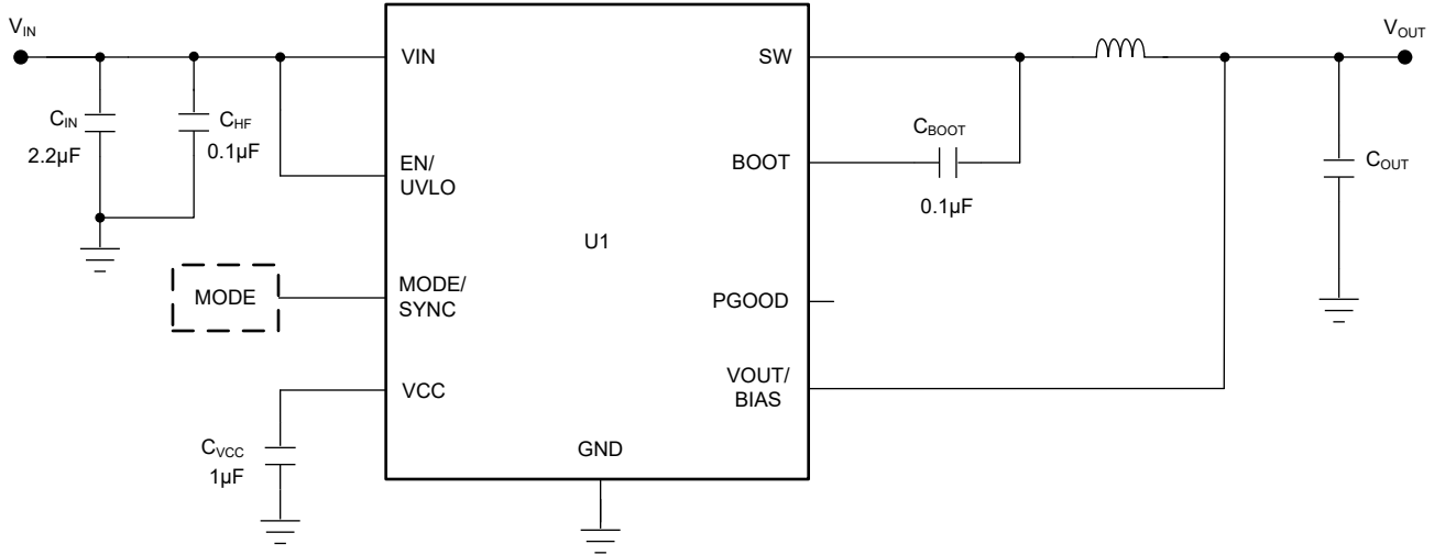
图 8-25. Schematic for Typical Application Curves
