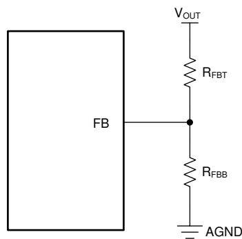
図 7-9. Setting Output Voltage for Adjustable Output Variant
