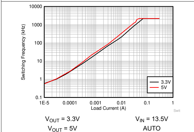
8-20. Switching Frequency Over Load Current
