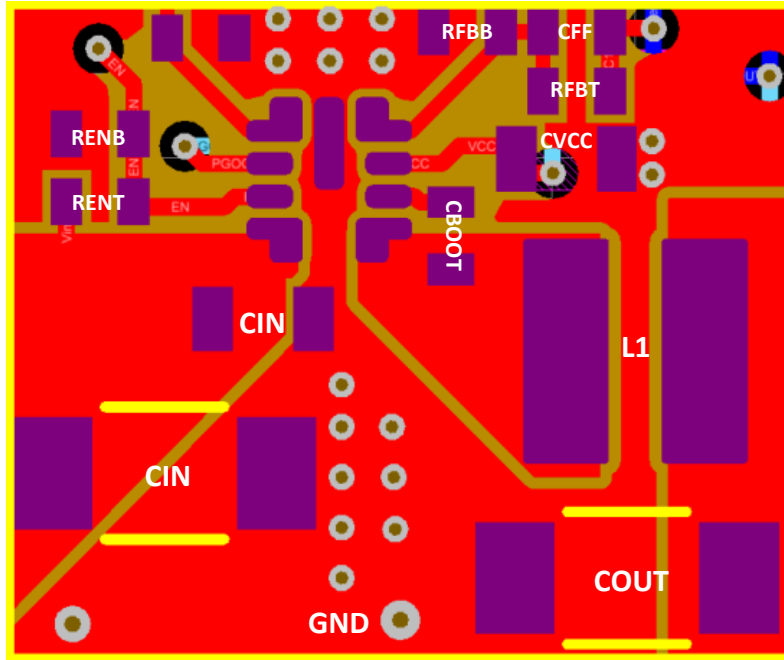
8-27. Example Layout
