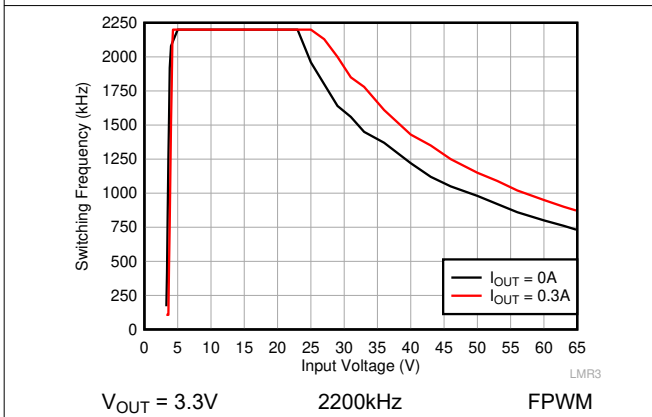
8-18. Switching Frequency over Input Voltage
