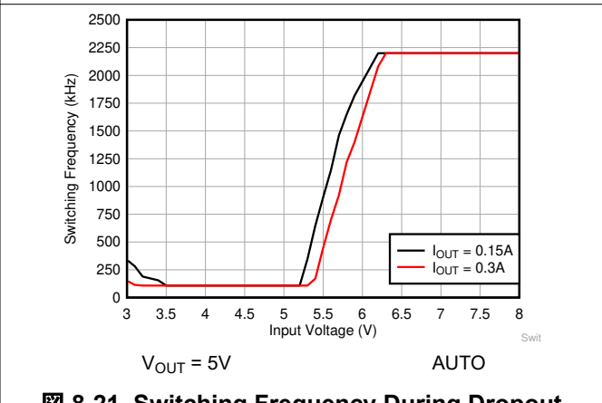
8-21. Switching Frequency During Dropout
