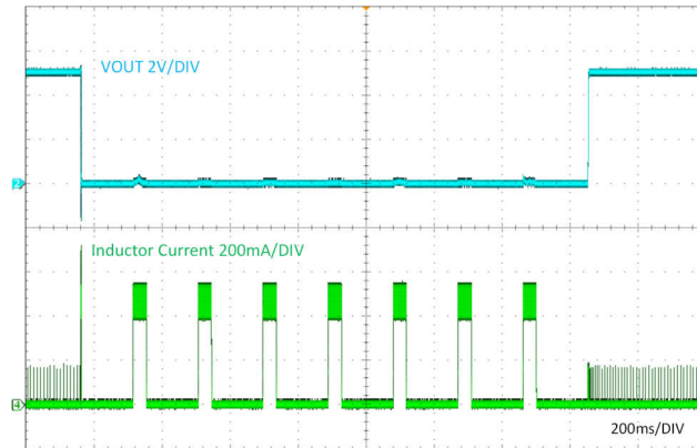
図 8-9. Short Protection and Recovery
