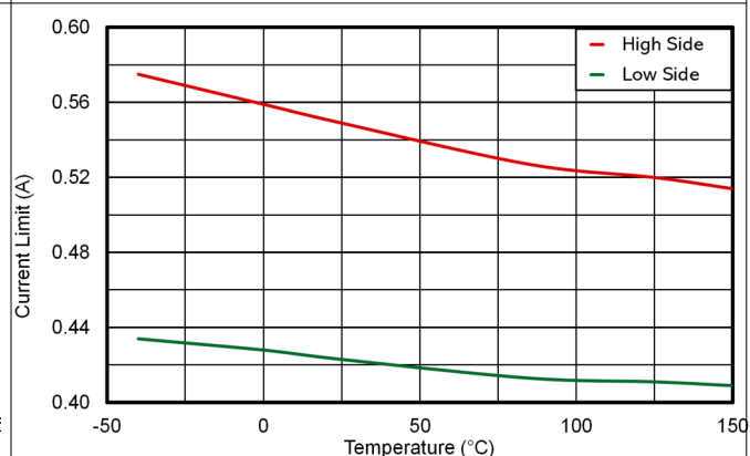
図 6-10. HS and LS Current Limit vs Temperature
