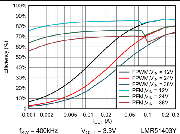
図 6-3. 3.3V Efficiency vs Load Current
