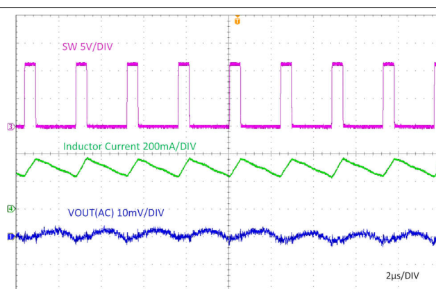
図 8-4. Ripple at Full Load
