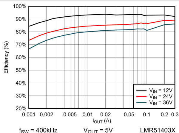
図 6-2. 5V Efficiency vs Load Current
