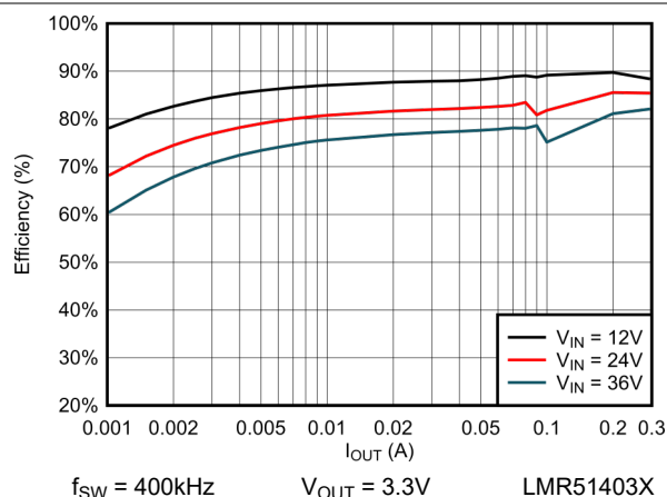
図 6-1. 3.3V Efficiency vs Load Current
