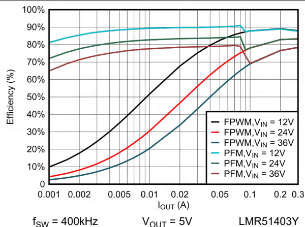
図 6-4. 5V Efficiency vs Load Current
