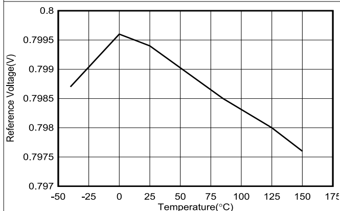
図 6-9. Reference Voltage vs Temperature
