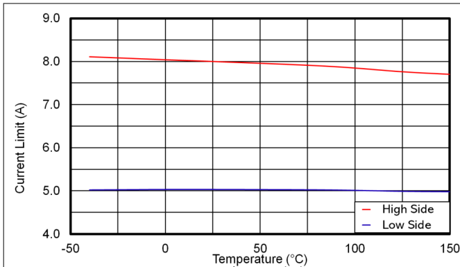
6-13. LMR51450-Q1 High Side and Low Side Current Limits
