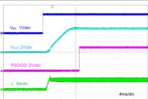
図 8-5. Start-Up by EN
