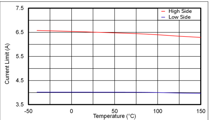
6-14. LMR51440-Q1 High Side and Low Side Current Limits
