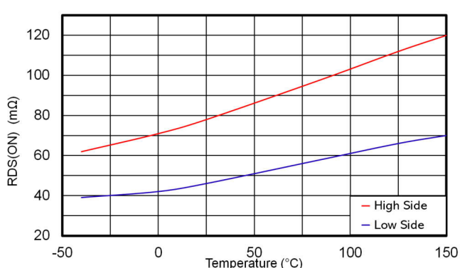
図 6-12. High Side and Low Side Switches R_{DS(on)}
