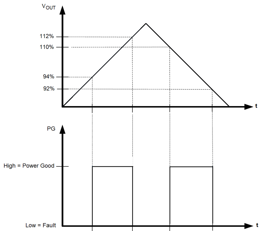
7-5. Static Power-Good Operation
