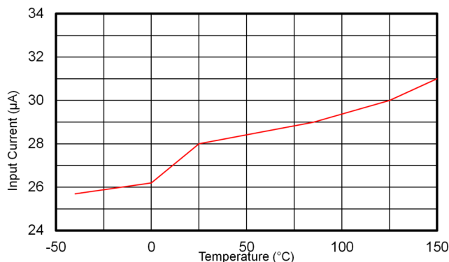
図 6-9. Non-Switching Input Supply Current
