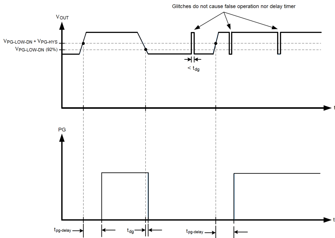
7-6. Power-Good Timing Behavior
