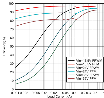
図 6-3. 5-V Efficiency Versus Load Current
