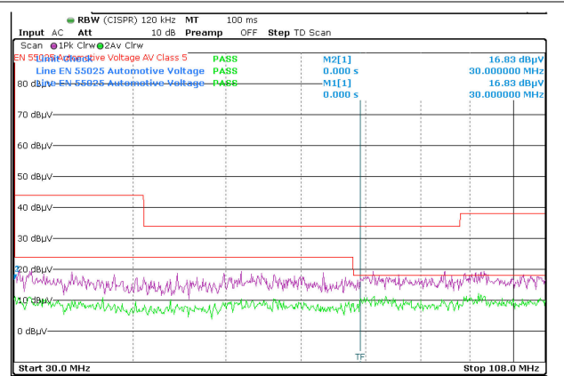
V_{OUT} = 3.3V F_{SW} = 2MHz I_{OUT} = 3A 測定周波数: 30MHz ~ 108MHz
