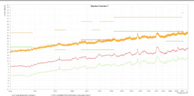
V_{OUT} = 3.3V F_{SW} = 2MHz I_{OUT} = 4A 測定周波数: 300MHz ~ 1GHz
