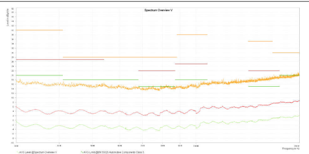
V_{OUT} = 3.3V F_{SW} = 2MHz I_{OUT} = 4A 測定周波数: 30MHz ~ 300MHz
