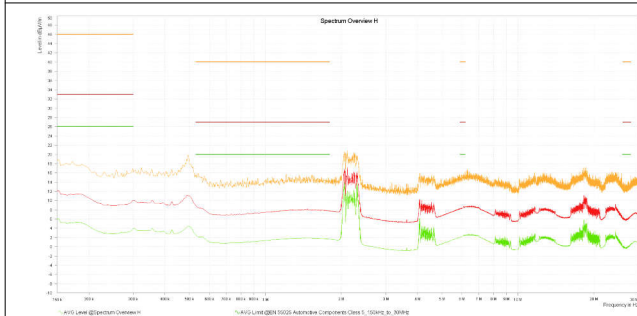
V_{OUT} = 3.3V F_{SW} = 2MHz I_{OUT} = 4A 測定周波数: 150kHz ~ 30MHz
