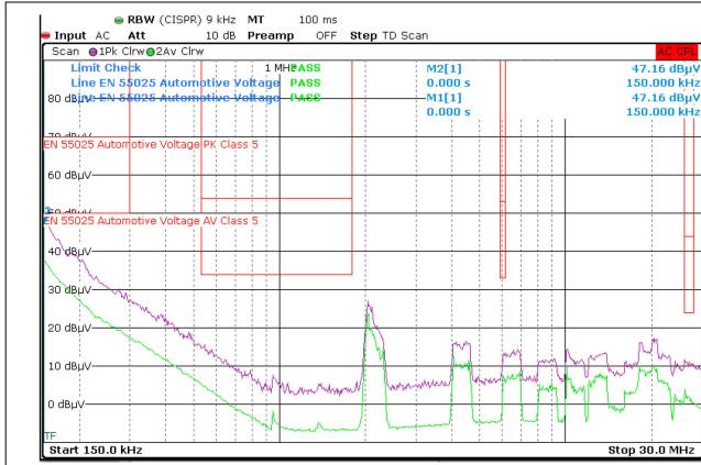
V_{OUT} = 3.3V F_{SW} = 2MHz I_{OUT} = 3A 測定周波数: 150kHz ~ 30MHz
