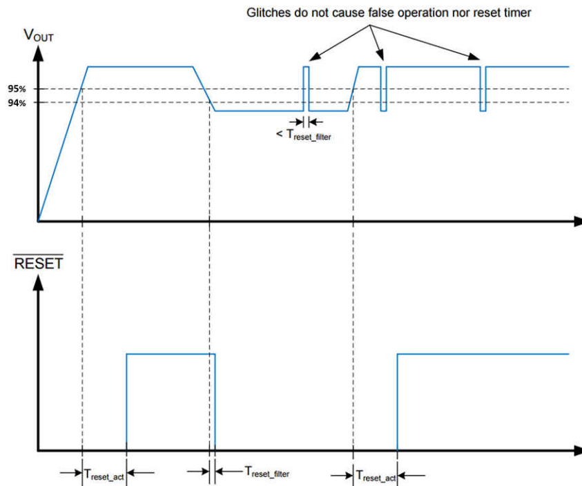
8-3. RESET Timing Behavior
