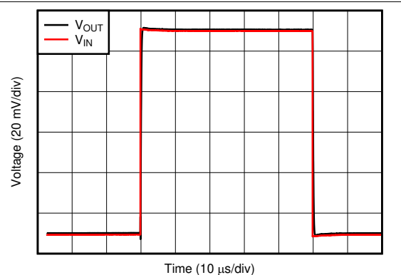
Figure 6-22. No Phase Reversal
