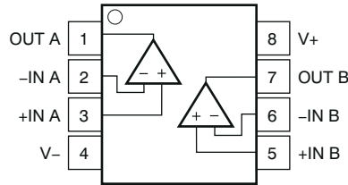
図 5-3. LMV358A-Q1 D and DGK Packages, 8-Pin SOIC and VSSOP (Top View)
