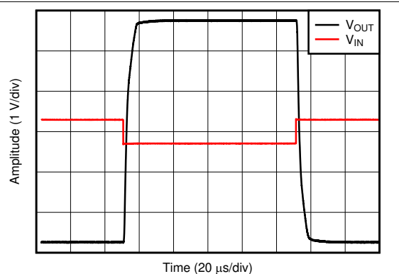
Figure 6-23. Overload Recovery
