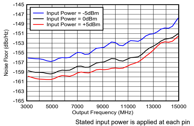
5-5. Noise Floor in Buffer Mode
