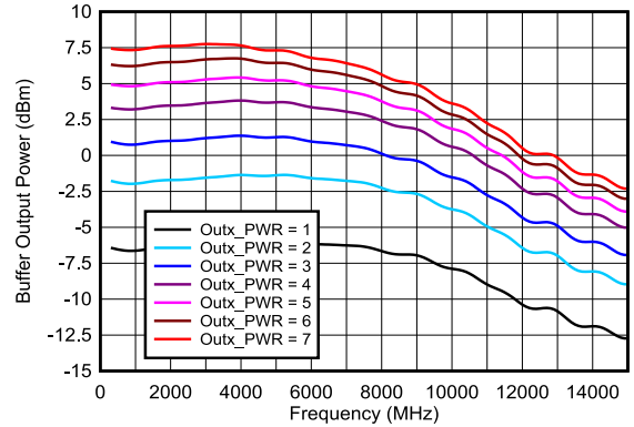
Applies to all modes except divider mode with odd divide (which have slightly lower power). 图 5-9. Buffer Mode Single-Ended Output Power
