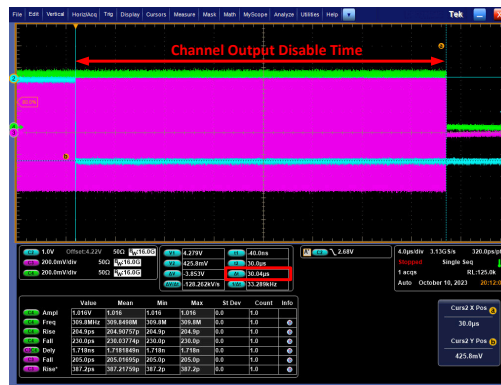
図 5-20. Channel Disable Setting Time
