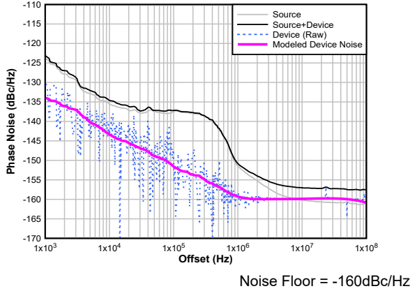
5-2. Buffer Phase Noise Plot at 6GHz Output
