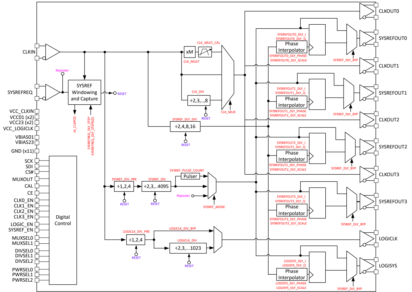
6-1. Functional Block Diagram
