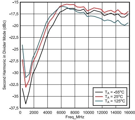
图 5-14. Second Harmonic on Divider Mode (Single-Ended Input)
