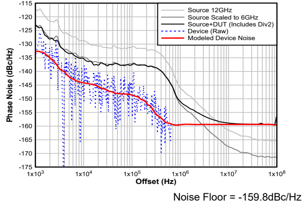
5-3. Divider Phase Noise Plot at 6GHz Output (Divide by 2)
