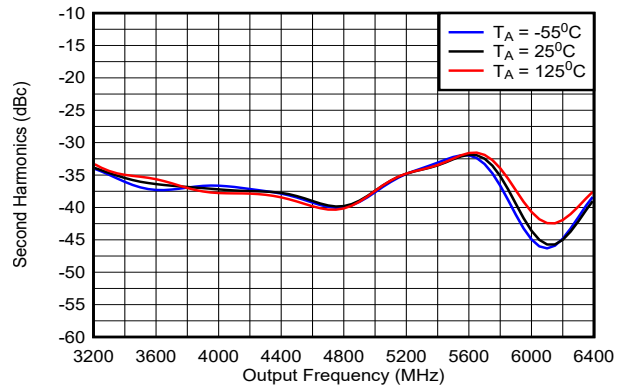
图 5-11. Second Harmonic in Multiply X2 Mode (Differential Output)
