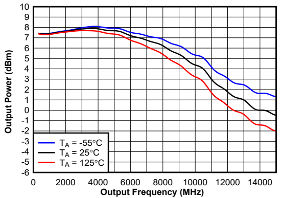
CLKOUTx_PWR = 7 图 5-10. Buffer Mode Single-Ended Output Power
