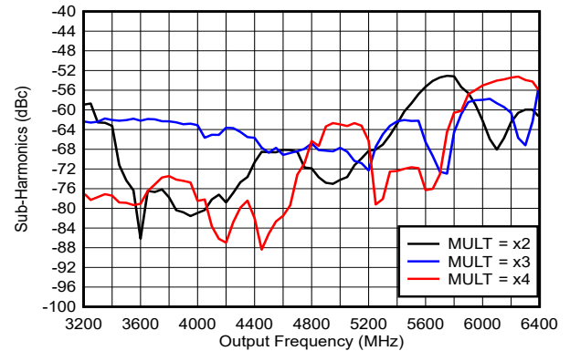
图 5-13. Multiplier Sub-Harmonics (Harmonic Frequency = Output Frequency / M)
