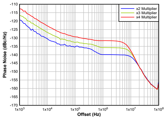
5-4. Multiplier Phase Noise Plot at 6GHz Output
