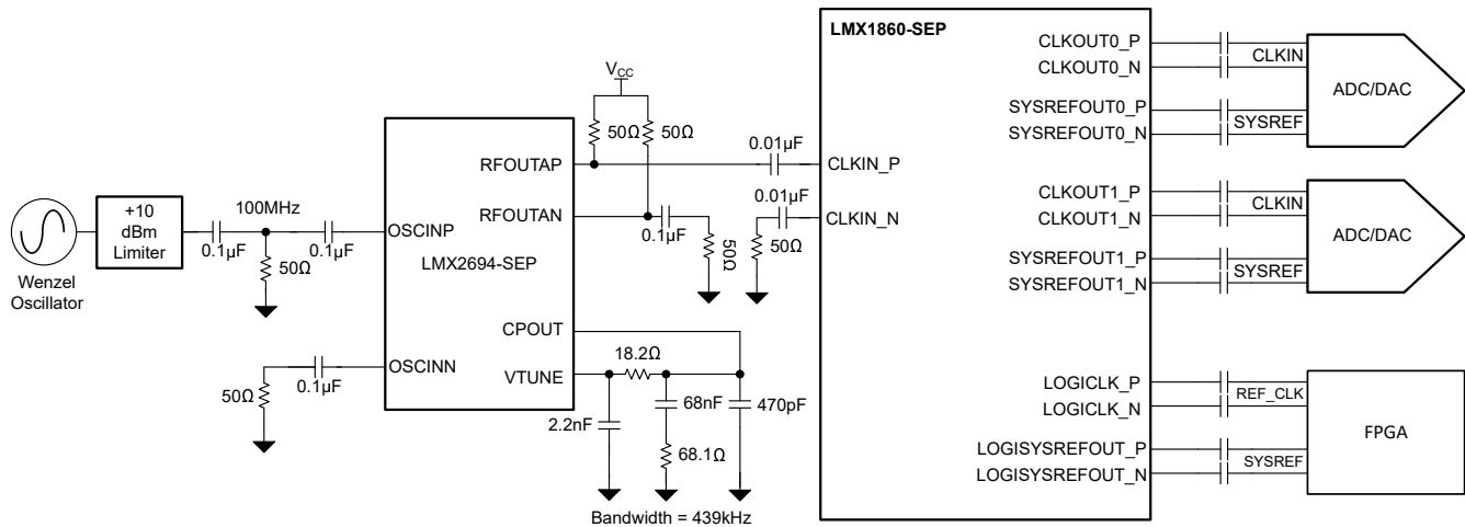
☒ 7-10. Typical JESD Clocks Block Diagram
