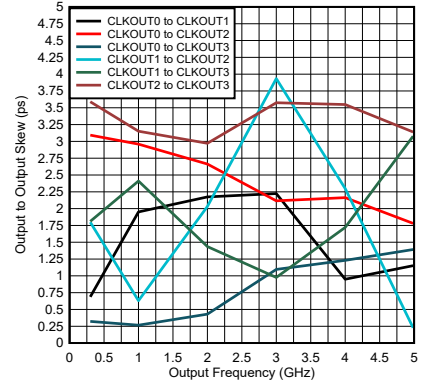
图 5-15. Output to Output Skew (ps)
