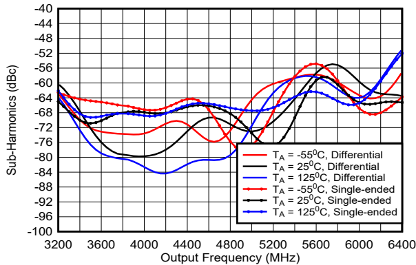
图 5-12. Multiplier 1/2 Sub-Harmonic in X2 Mode
