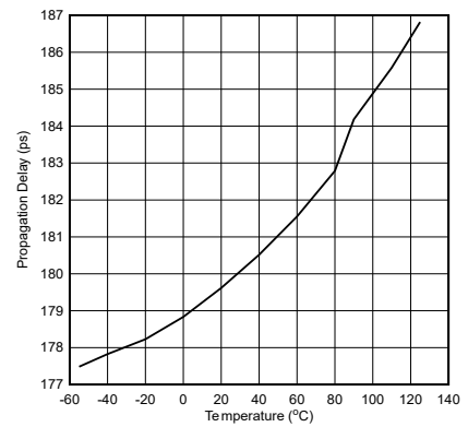
图 5-18. Propagation Delay
