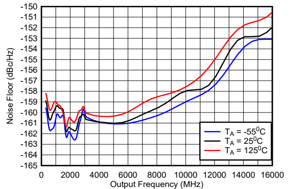
5-7. Noise Floor in Buffer Mode
