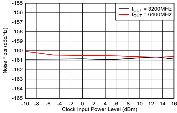
Input is differential 图 5-8. Noise Floor in Multiply x2 Mode
