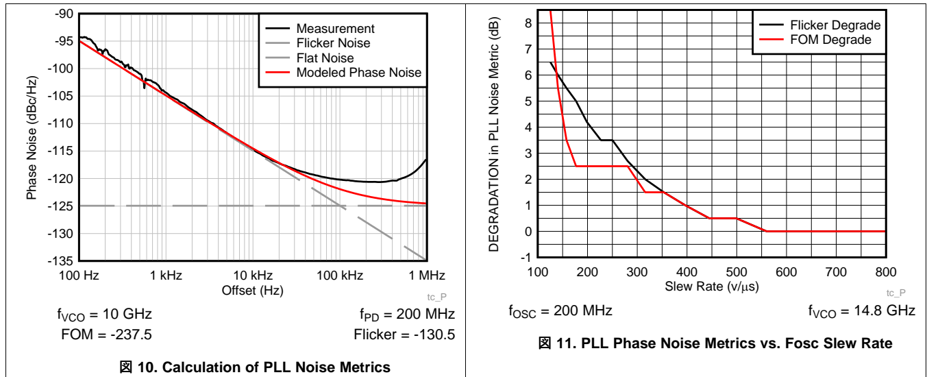
Figure 10. Calculation of PLL Noise Metrics
