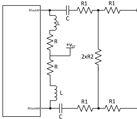
75. Termination of Unused Output
