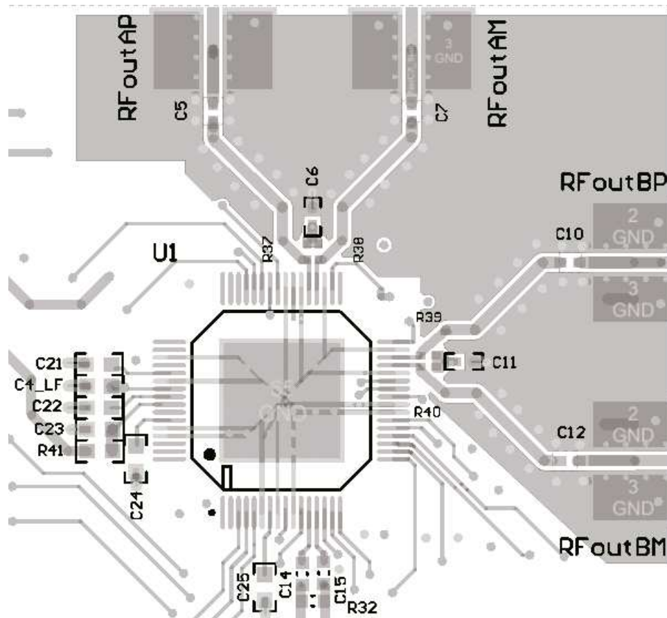
79. LMX2615 Layout Example
