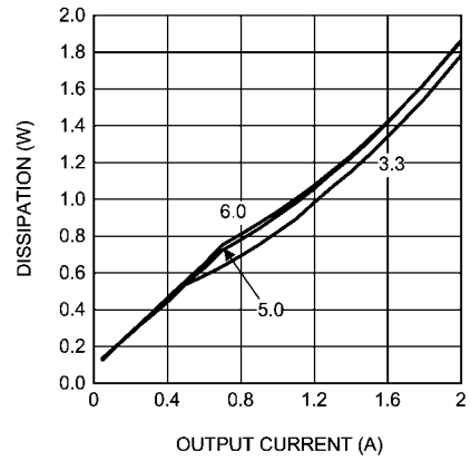
Dissipation 36V input @ 85°C
