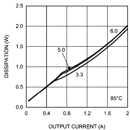
Dissipation 42V Input @ 85°C
