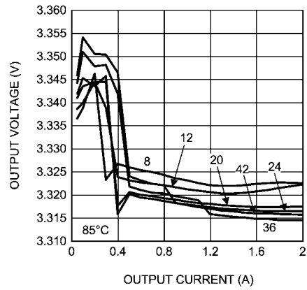
Line and Load Regulation @ 85°C
