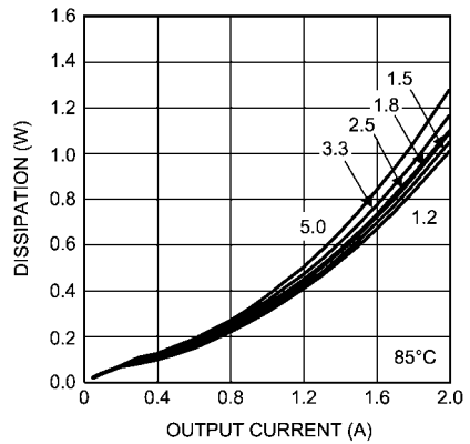
Dissipation 8V input 85°C
