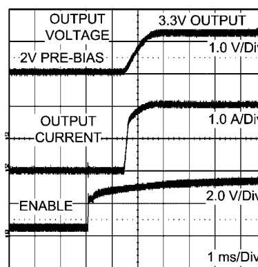
Pre-biased startup
