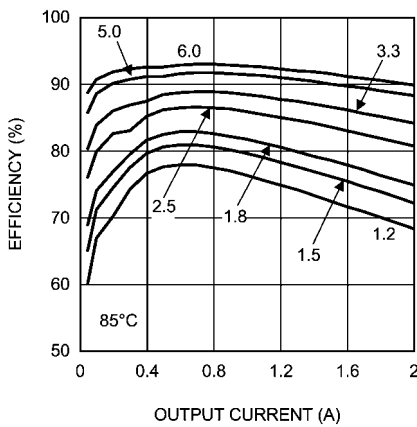
Efficiency 12V input @ 85°C
