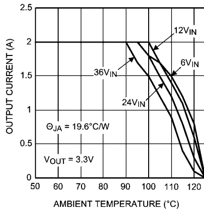
Thermal Derating V OUT = 3.3V
