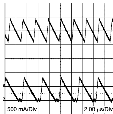
CCM and DCM Operating Modes V IN = 24V, V O = 3.3V, I O = 3A/0.4A 2 μsec/div
