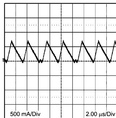
Transition Mode Operation V IN = 24V, V O = 3.3V, I O = 0.5 A 2 μsec/div
