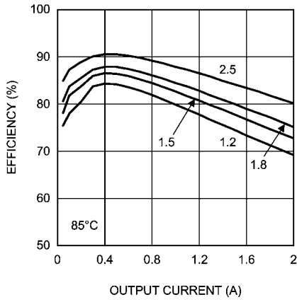
Efficiency 6V Input @ 85°C
