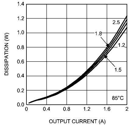
Dissipation 6V input @ 85°C
