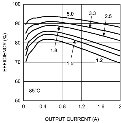
Efficiency 8V input 85°C
