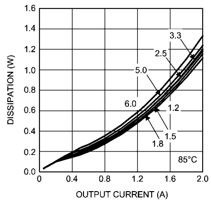
Dissipation 12V input @ 85°C
