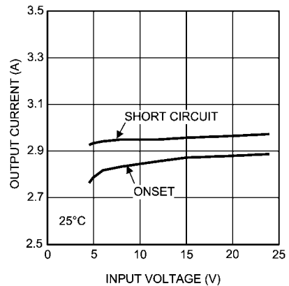
Current Limit 1.8V OUT @ 25°C
