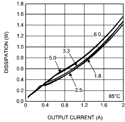
Dissipation 24V input @ 85°C
