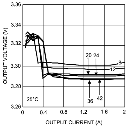
Line and Load Regulation @ 25°C
