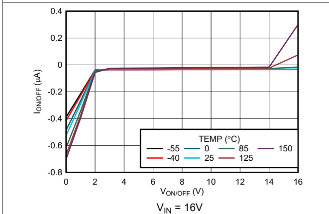
図 5-39. \text{ON}/\overline{\text{OFF}} Pin Current vs V_{\text{ON}/\overline{\text{OFF}}} (New Chip)
