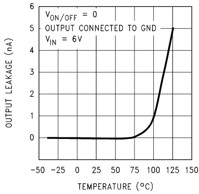
5-31. Input to Output Leakage vs Temperature (Legacy Chip)
