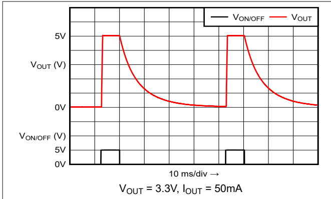
図 5-37. Turnoff Waveform (New Chip)
