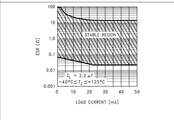
図 5-42. 2.2\mu\text{F} ESR Range vs I_{\text{OUT}} (Legacy Chip)
