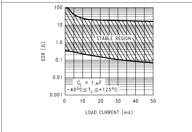
図 5-41. 1\mu\text{F} ESR Range vs I_{\text{OUT}} (Legacy Chip)
