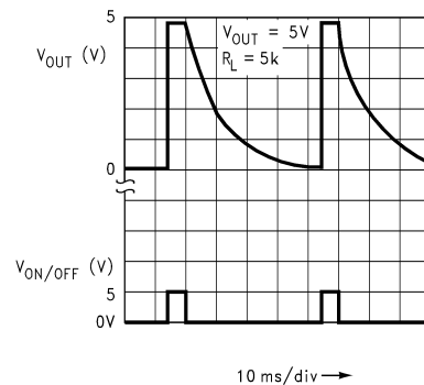
5-34. Turn-On Waveform (Legacy Chip)
