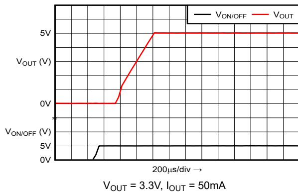
5-35. Turn-On Waveform (New Chip)
