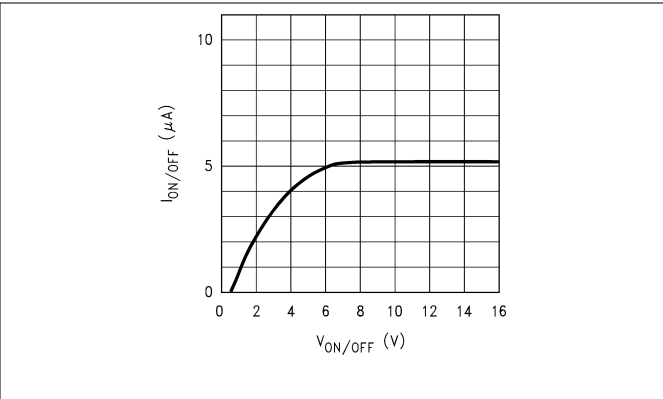
図 5-38. \text{ON}/\overline{\text{OFF}} Pin Current vs V_{\text{ON}/\overline{\text{OFF}}} (Legacy Chip)
