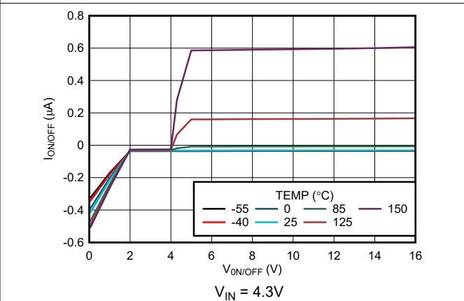
図 5-40. \text{ON}/\overline{\text{OFF}} Pin Current vs V_{\text{ON}/\overline{\text{OFF}}} (New Chip)
