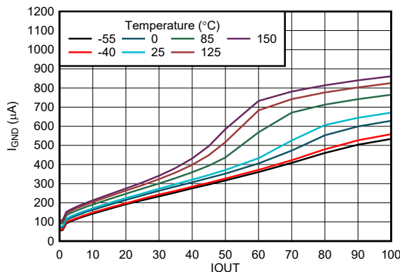
5-11. Ground Pin Current ( I_{GND} ) vs Load Current (New Chip)
