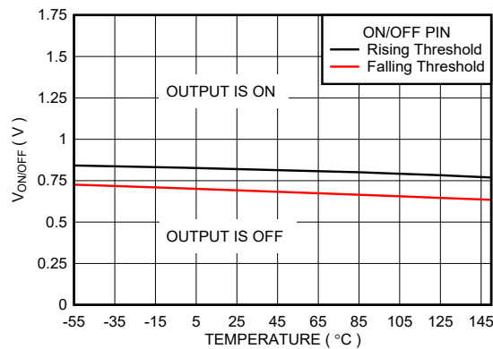
5-29. ON/ OFF Threshold vs Temperature (New Chip)
