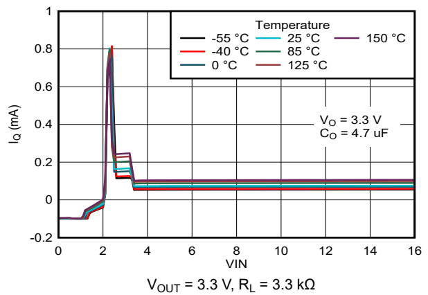
5-12. Input Current vs Input Voltage ( V_{IN} ) (New Chip)
