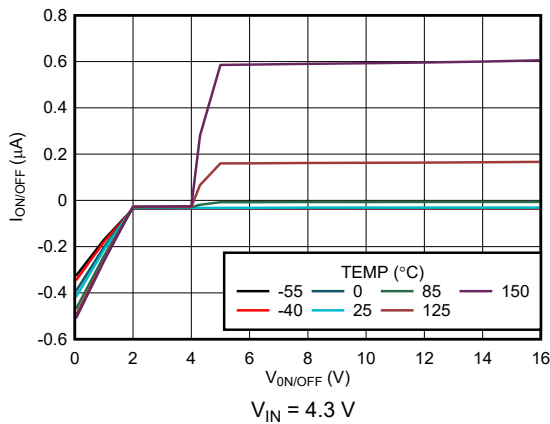
5-27. ON/ OFF Pin Current vs V_{ON/OFF} (New Chip)
