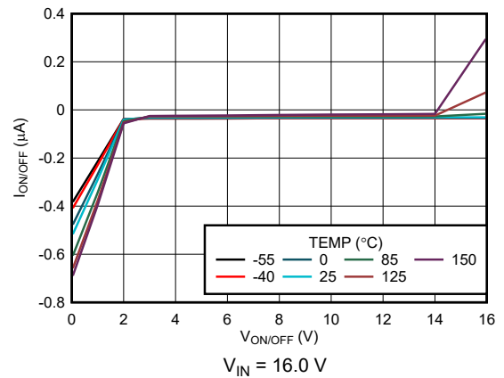
5-28. ON/ OFF Pin Current vs V_{ON/OFF} (New Chip)
