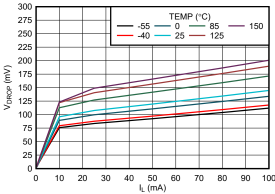
5-9. Dropout Voltage ( V_{DO} ) vs Load Current (New Chip)
