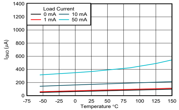
5-10. Ground Pin Current ( I_{GND} ) vs Temperature (New Chip)
