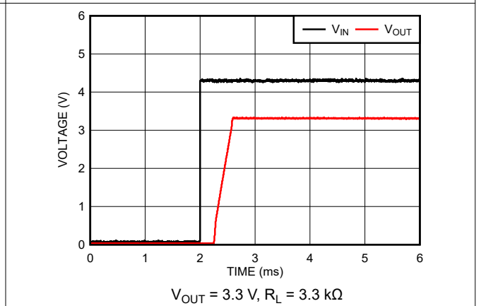
7-10. Turn-on Waveform (New Chip)
