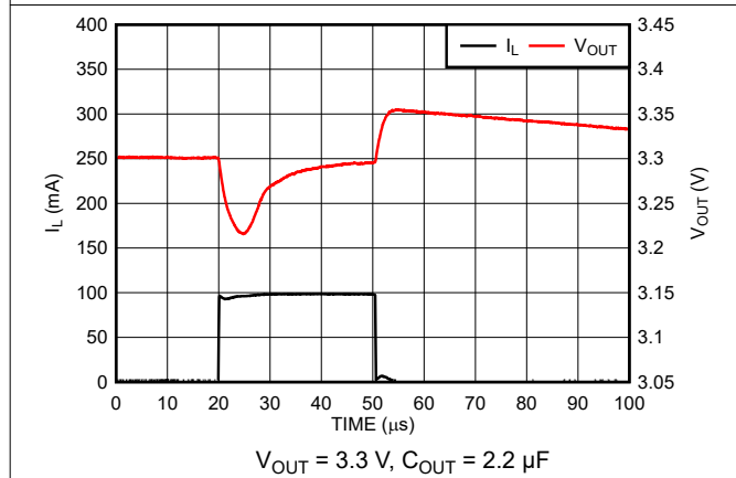
7-9. Load Transient Response (New Chip)
