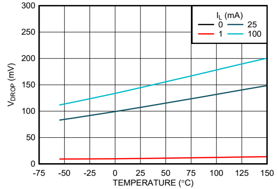
5-8. Dropout Voltage ( V_{DO} ) vs Temperature (New Chip)
