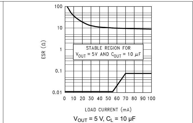
図 7-4. 5-V, 10- \mu F ESR Curves (Legacy Chip)
