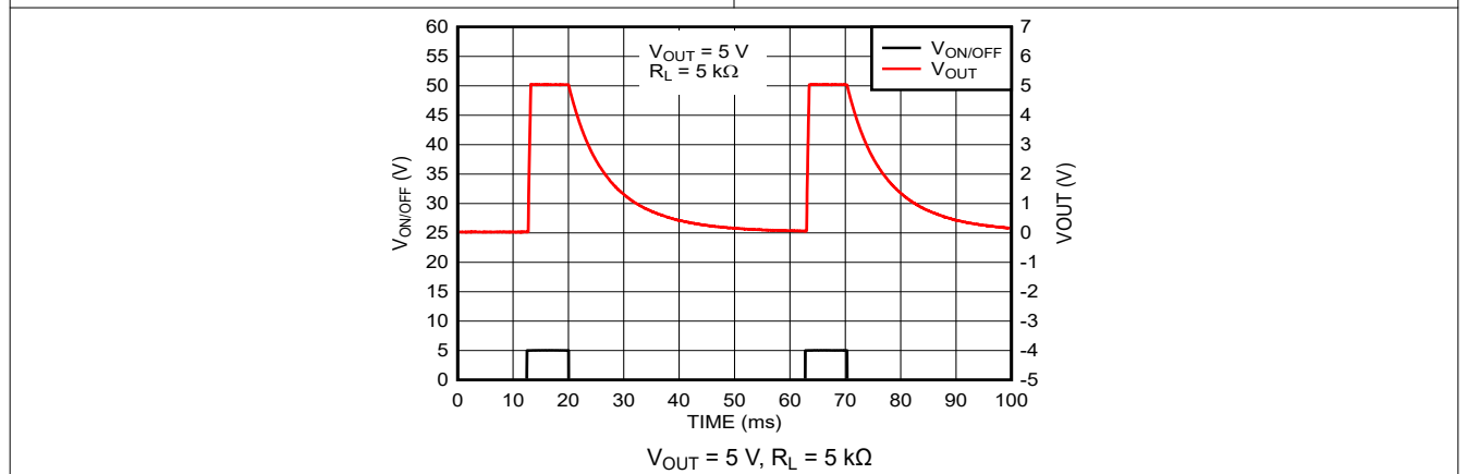
7-11. Turn-off Waveform (New Chip)
